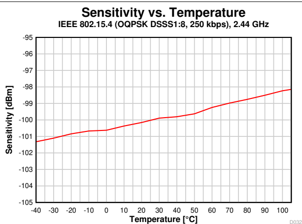
7-13. Sensitivity vs. Temperature (250 kbps, 2.44 GHz)
