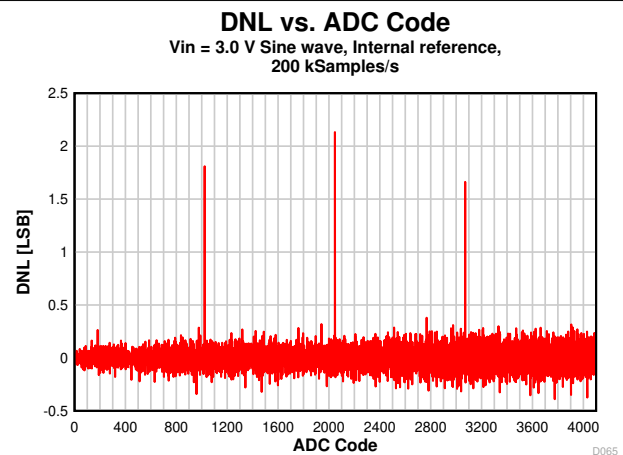
7-26. DNL vs. ADC Code
