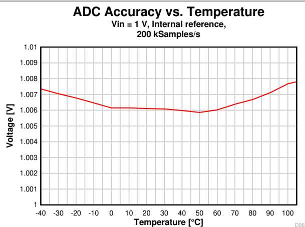
7-27. ADC Accuracy vs. Temperature
