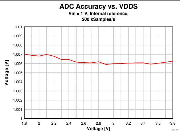
7-28. ADC Accuracy vs. Supply Voltage (VDD)
