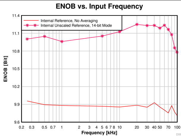
7-23. ENOB vs. Input Frequency
