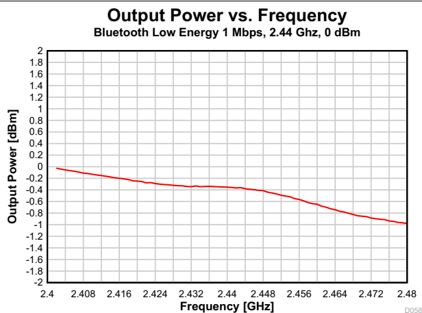
FIG 7-21. Output Power vs. Frequency (Bluetooth Low Energy 1 Mbps, 2.44 GHz)
