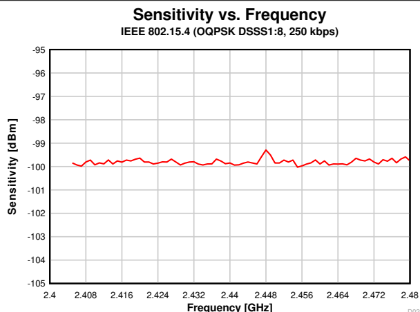
7-11. Sensitivity vs. Frequency (250 kbps, 2.44 GHz)
