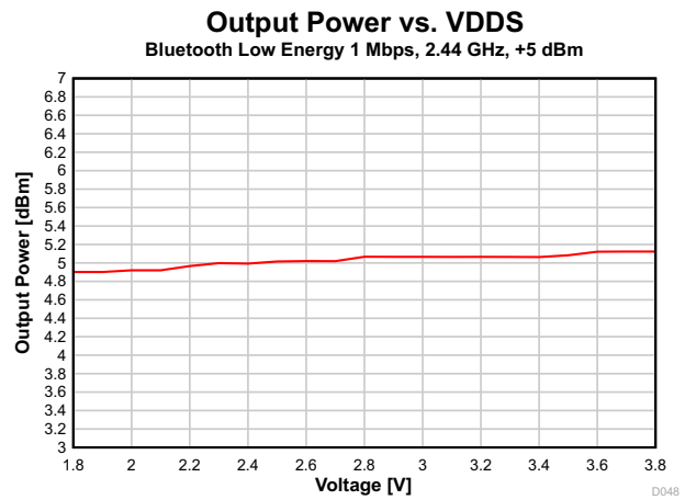
FIG 7-20. Output Power vs. Supply Voltage (VDD5) (Bluetooth Low Energy 1 Mbps, 2.44 GHz, +5 dBm)
