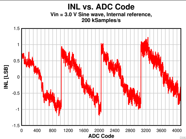
7-25. INL vs. ADC Code
