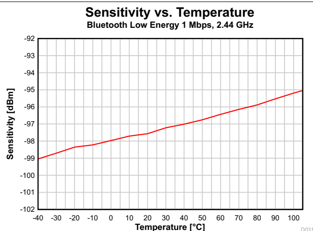
7-12. Sensitivity vs. Temperature (Bluetooth Low Energy 1 Mbps, 2.44 GHz)
