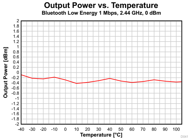
FIG 7-17. Output Power vs. Temperature (Bluetooth Low Energy 1 Mbps, 2.44 GHz)
