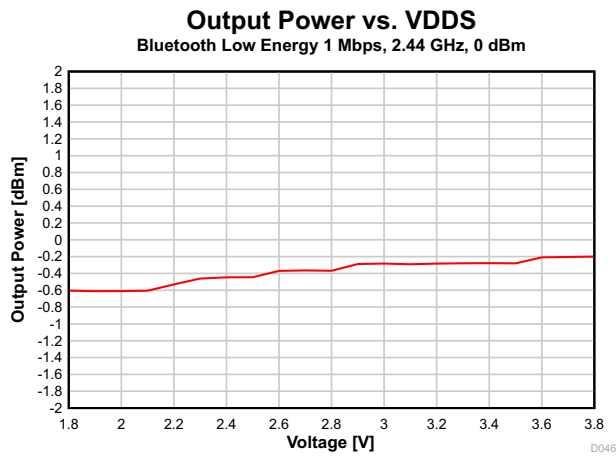
FIG 7-19. Output Power vs. Supply Voltage (VDD5) (Bluetooth Low Energy 1 Mbps, 2.44 GHz)
