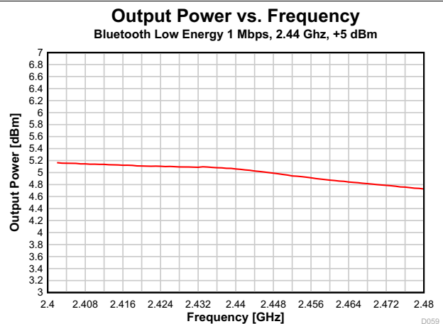
FIG 7-22. Output Power vs. Frequency (Bluetooth Low Energy 1 Mbps, 2.44 GHz, +5 dBm)
