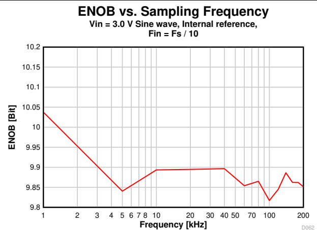
7-24. ENOB vs. Sampling Frequency
