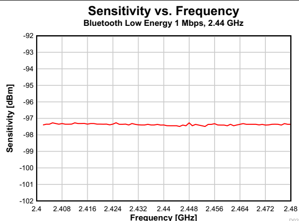
7-10. Sensitivity vs. Frequency (Bluetooth Low Energy 1 Mbps, 2.44 GHz)
