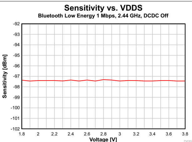
7-15. Sensitivity vs. Supply Voltage (VDD) (Bluetooth Low Energy 1 Mbps, 2.44 GHz, DCDC Off)
