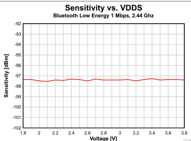
7-14. Sensitivity vs. Supply Voltage (VDD) (Bluetooth Low Energy 1 Mbps, 2.44 GHz)
