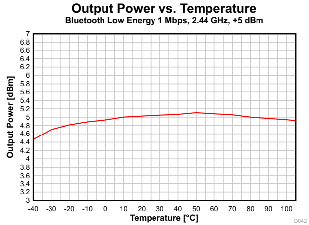
FIG 7-18. Output Power vs. Temperature (Bluetooth Low Energy 1 Mbps, 2.44 GHz, +5 dBm)
