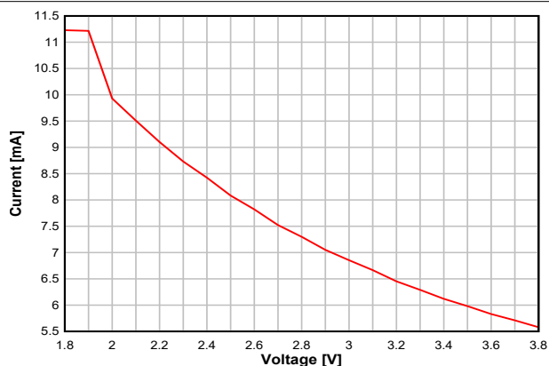
図 8-7. RX Current vs. Supply Voltage (VDDS) (BLE 1 Mbps, 2.44 GHz)
