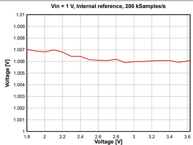
8-35. ADC Accuracy vs. Supply Voltage (VDD5)
