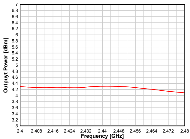
8-28. Output Power vs. Frequency (BLE 1 Mbps, +5 dBm)
