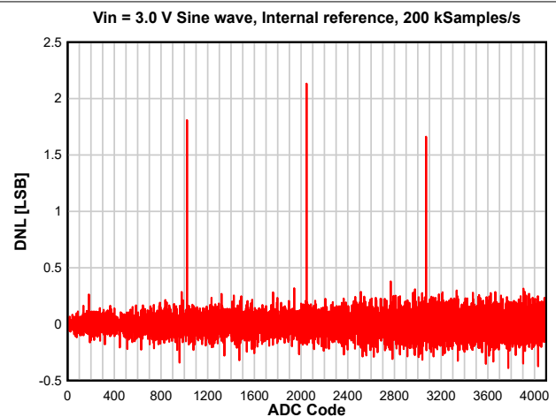
8-33. DNL vs. ADC Code
