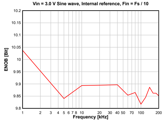
8-31. ENOB vs. Sampling Frequency
