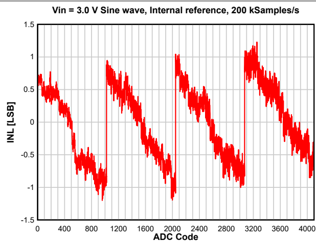
8-32. INL vs. ADC Code
