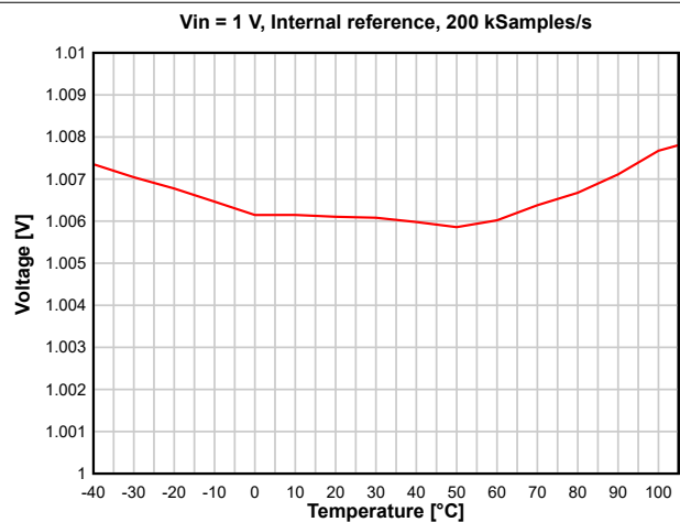
8-34. ADC Accuracy vs. Temperature
