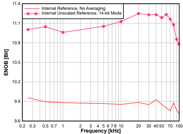
8-30. ENOB vs. Input Frequency
