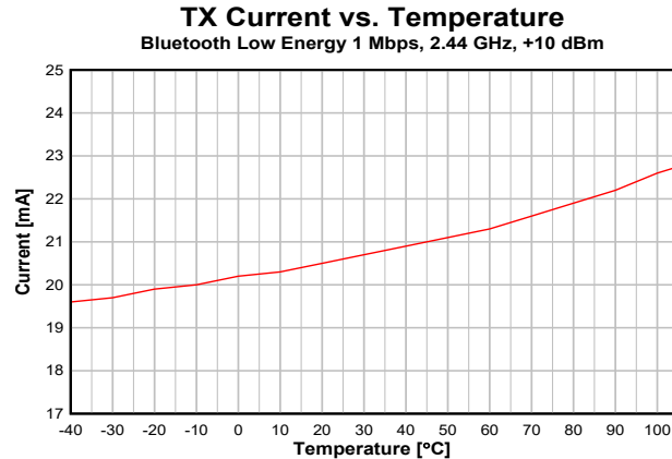
8-8. TX Current vs. Temperature (BLE 1 Mbps, 2.44 GHz)
