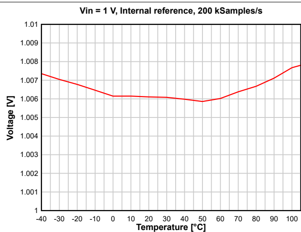
8-26. ADC Accuracy versus Temperature
