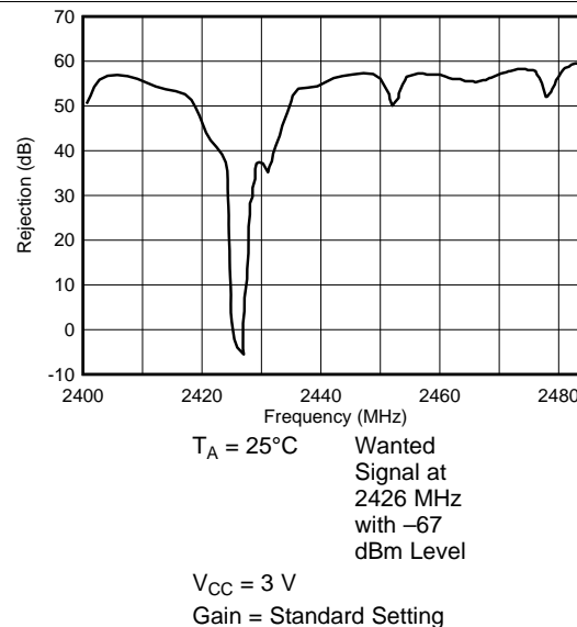
Figure 4-16. RX Interferer Rejection (Selectivity) vs Interferer Frequency
