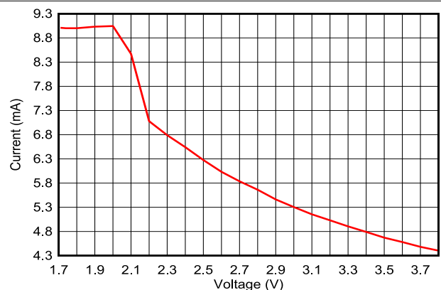
Figure 7-12. TX Current vs. Supply Voltage, VDD (BLE 1Mbps, 2.44GHz, 0dBm)
