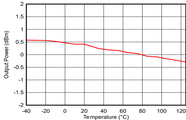
FIG 7-21. Output Power vs. Temperature (BLE 1Mbps, 2.44GHz, 0dBm)
