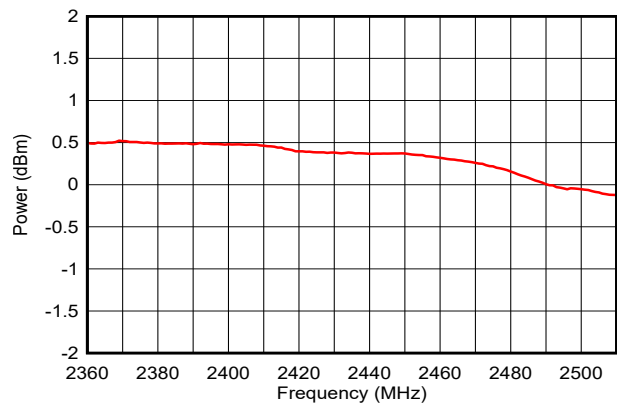
FIG 7-25. Output Power vs. Frequency (BLE 1Mbps, 0dBm)
