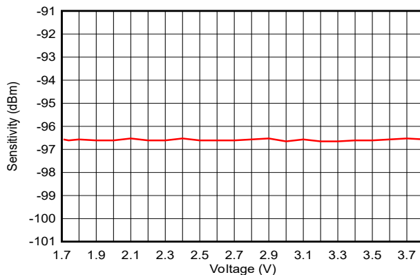
図 7-20. Sensitivity vs. Supply Voltage (VDD) (BLE 1Mbps, 2.44GHz, DCDC Off)
