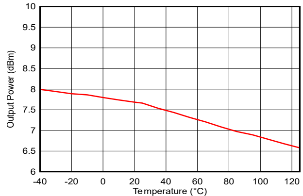
FIG 7-22. Output Power vs. Temperature (BLE 1Mbps, 2.44GHz, +8dBm)
