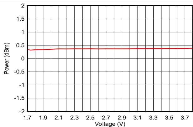
FIG 7-23. Output Power vs. Supply Voltage (VDD5) (BLE 1Mbps, 2.44GHz, 0dBm)
