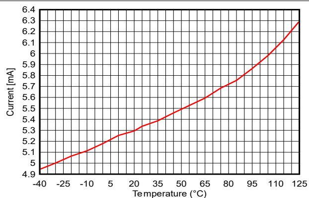
図 7-8. RX Current vs. Temperature (BLE 1Mbps, 2.44GHz)
