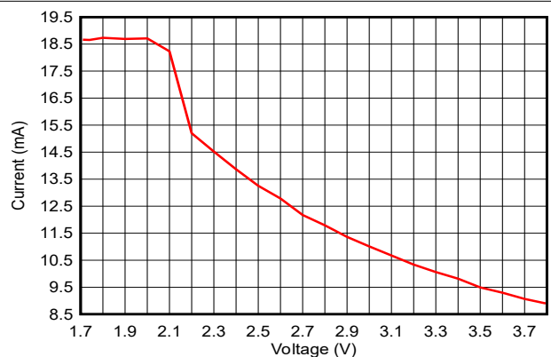
Figure 7-13. TX Current vs. Supply Voltage, VDD (BLE 1Mbps, 2.44GHz, +8dBm)
