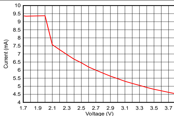
図 7-9. RX Current vs. Supply Voltage (VDD) (BLE 1Mbps, 2.44GHz)
