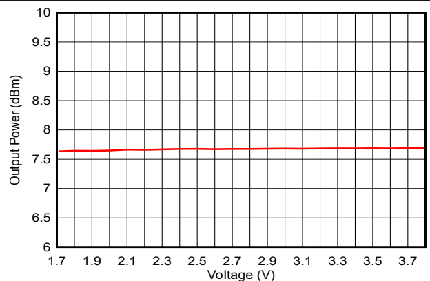
FIG 7-24. Output Power vs. Supply Voltage (VDD5) (BLE 1Mbps, 2.44GHz, +8dBm)
