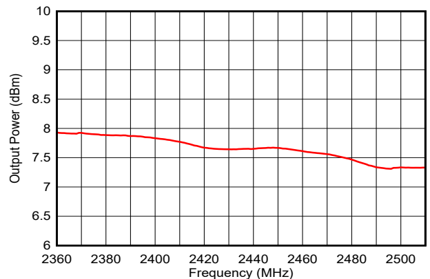
FIG 7-26. Output Power vs. Frequency (BLE 1Mbps, +8dBm)
