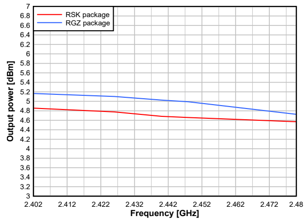
図 7-34. Output Power vs. Frequency (BLE 1Mbps, 2.44GHz, +5dBm)
