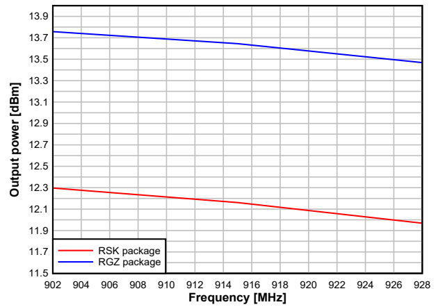
図 7-32. Output Power vs. Frequency (50kbps, 915MHz, +14dBm)
