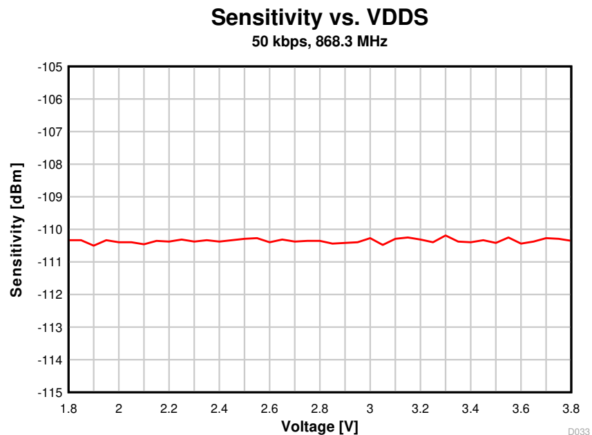
8-24. Sensitivity vs. Supply Voltage (VDD) (50 kbps, 868.3 MHz)
