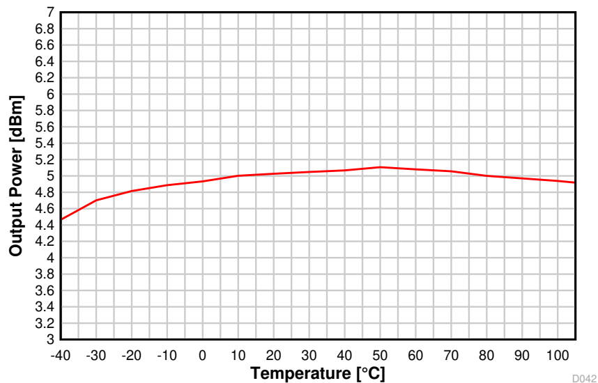
8-35. Output Power vs. Temperature (BLE 1 Mbps, 2.44 GHz, +5 dBm)
