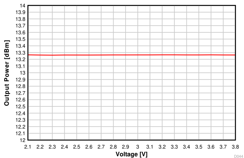
8-36. Output Power vs. Supply Voltage (VDD5) (50 kbps, 868.3 MHz)
