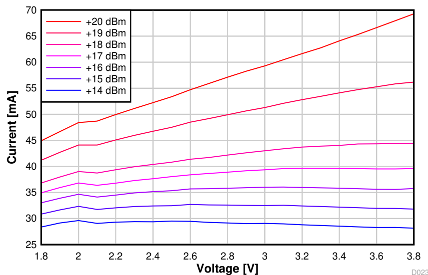
8-19. TX Current vs. Supply Voltage (VDD5) (50 kbps, 915 MHz)
