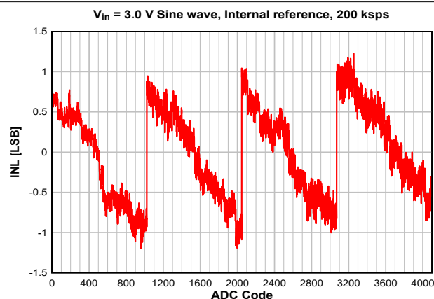
7-21. INL vs. ADC Code
