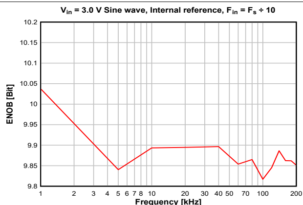
7-20. ENOB vs. Sampling Frequency
