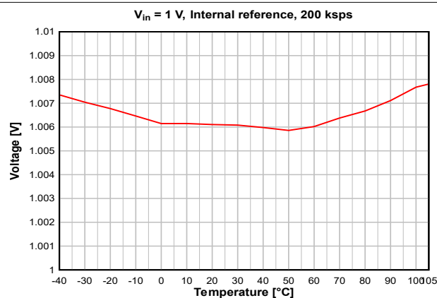
7-23. ADC Accuracy vs. Temperature
