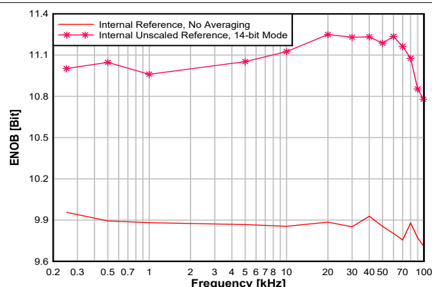
7-19. ENOB vs. Input Frequency
