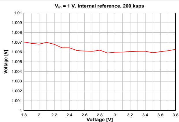
7-24. ADC Accuracy vs. Supply Voltage (VDD)
