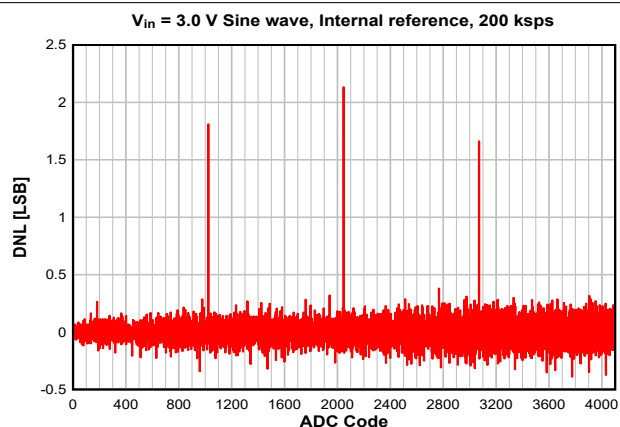
7-22. DNL vs. ADC Code
