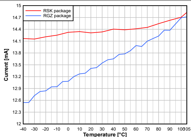
図 7-8. TX Current vs. Temperature (50kbps, 868.3MHz, +10dBm, VDDS = 3.6V)
