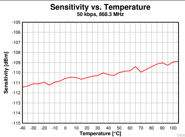
7-12. Sensitivity vs. Temperature (50 kbps, 868.3 MHz)
