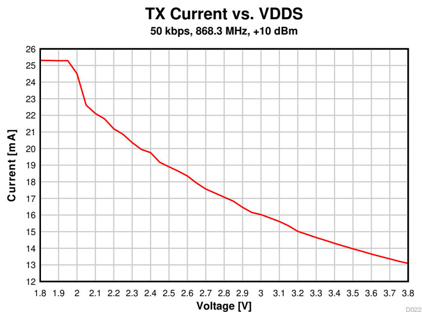
8-11. TX Current vs. Supply Voltage (VDD) (50 kbps, 868.3 MHz)
