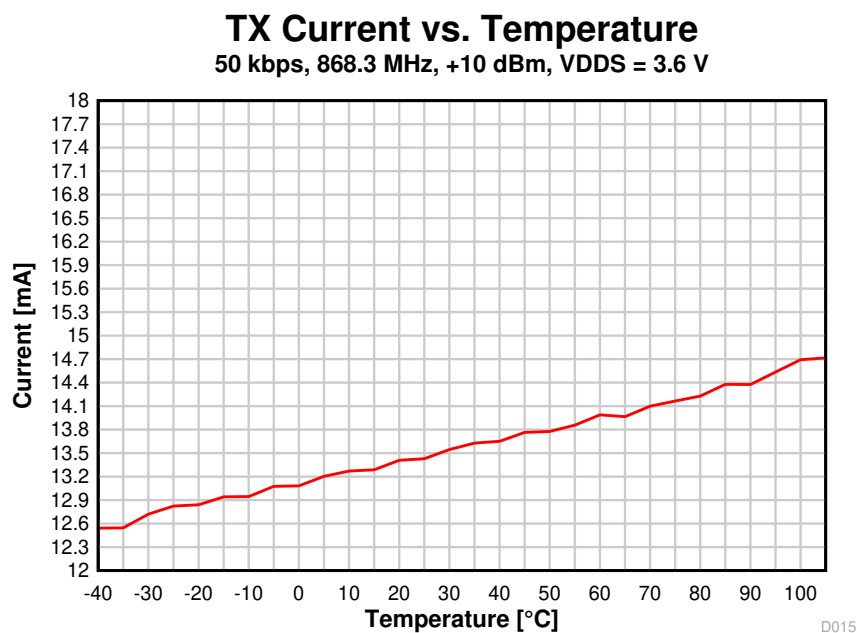
8-10. TX Current vs. Temperature (50 kbps, 868.3 MHz, VDD = 3.6 V)
