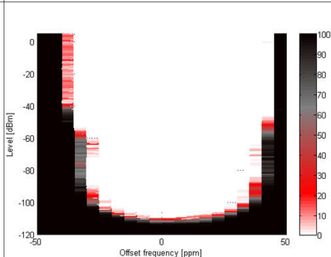
8-17. 802.15.4, 50 kbps, ±25 kHz deviation, 2-GFSK, 100 kHz RX Bandwidth
