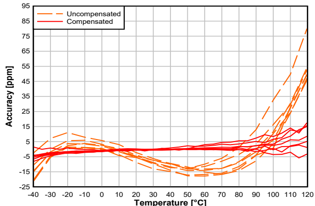
8-32. Temperature Compensation of the RF Frequency
