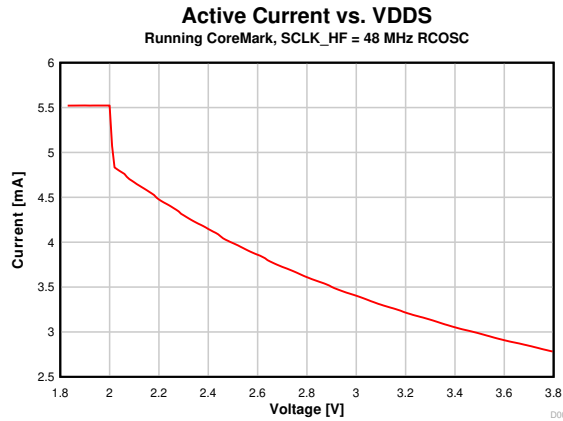
図 8-4. Active Mode (MCU) Current vs. Supply Voltage (VDD) (Running CoreMark, SCLK_HF = 48 MHz RCOSC)
