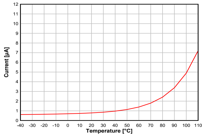
図 8-6. Standby Mode (MCU) Current vs. Temperature, 80kB RAM retention, no Cache retention, RTC On SCLK_LF = 32 kHz XOSC, VDD = 3.6 V
