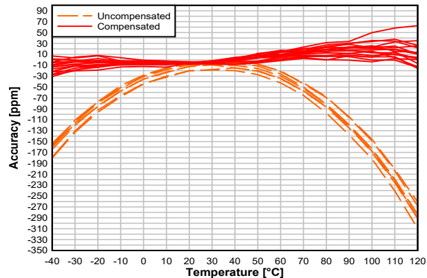
8-31. Temperature Compensation of the Real Time Clock (RTC)
