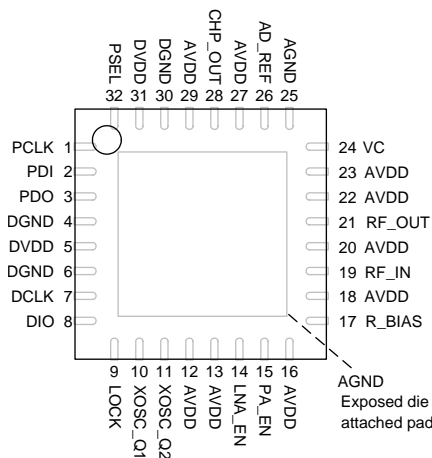
Figure 3-1. Package 7-mm × 7-mm VQFNP (Top View)
