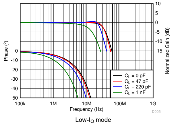
Figure 6-23. Gain and Phase vs Frequency and Load Capacitance
