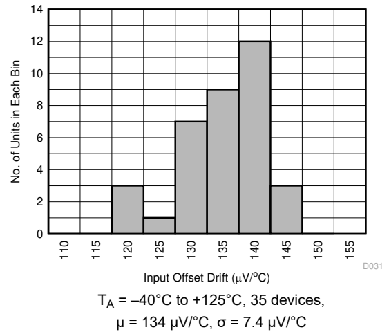
図 6-44. Offset Voltage Drift Distribution Histogram
