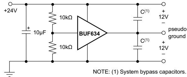
8-3. Pseudo-Ground Driver
