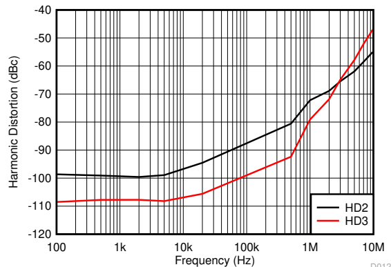
Wide-BW mode, V_{IN} = 10\text{ V}_{PP} , R_L = 1\text{ k}\Omega Figure 6-29. Harmonic Distortion vs Frequency
