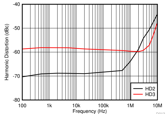
Wide-BW mode, V_{IN} = 10\text{ V}_{PP} , R_L = 100\ \Omega Figure 6-30. Harmonic Distortion vs Frequency
