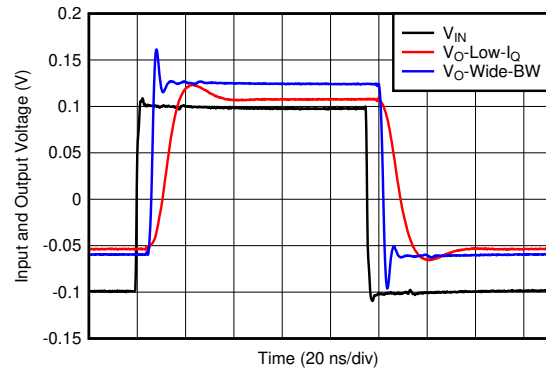
図 6-38. Small-Signal Transient Response
