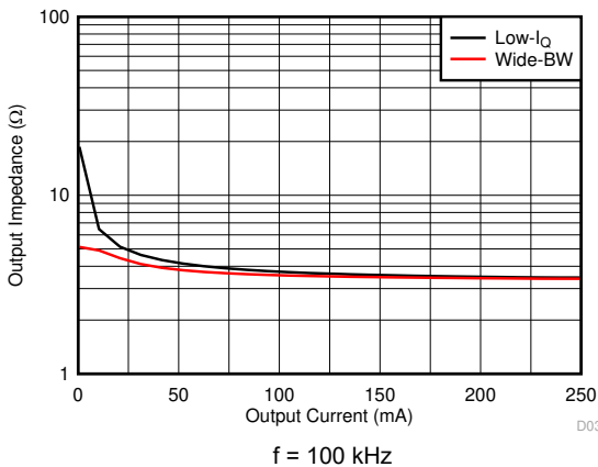
図 6-39. Output Impedance vs Output Current
