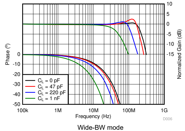
Figure 6-24. Gain and Phase vs Frequency and Load Capacitance
