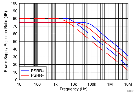
Solid lines indicate wide-BW mode, dashed lines indicate low- I_Q mode Figure 6-26. PSRR vs Frequency
