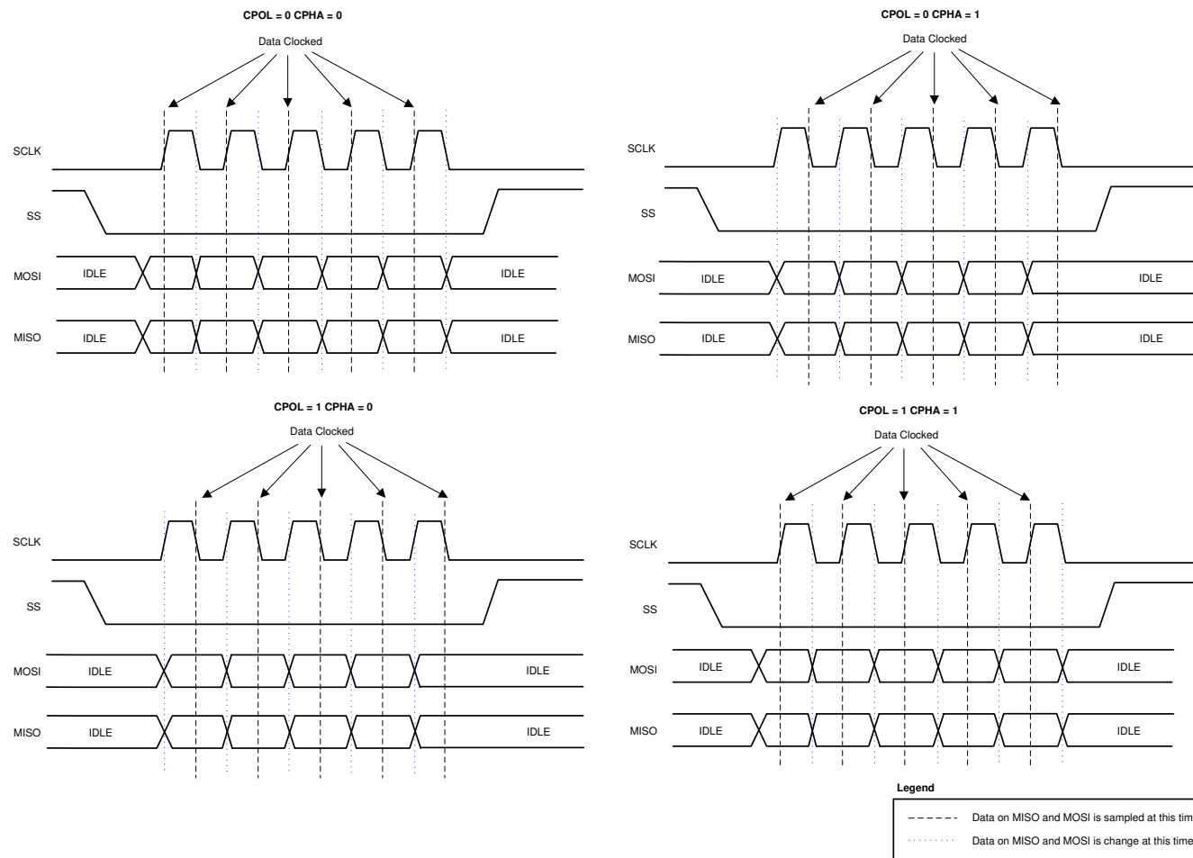
図 8-33. SPI Master CPOL and CPHA
