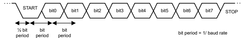
図 8-16. UART Communication to Host
