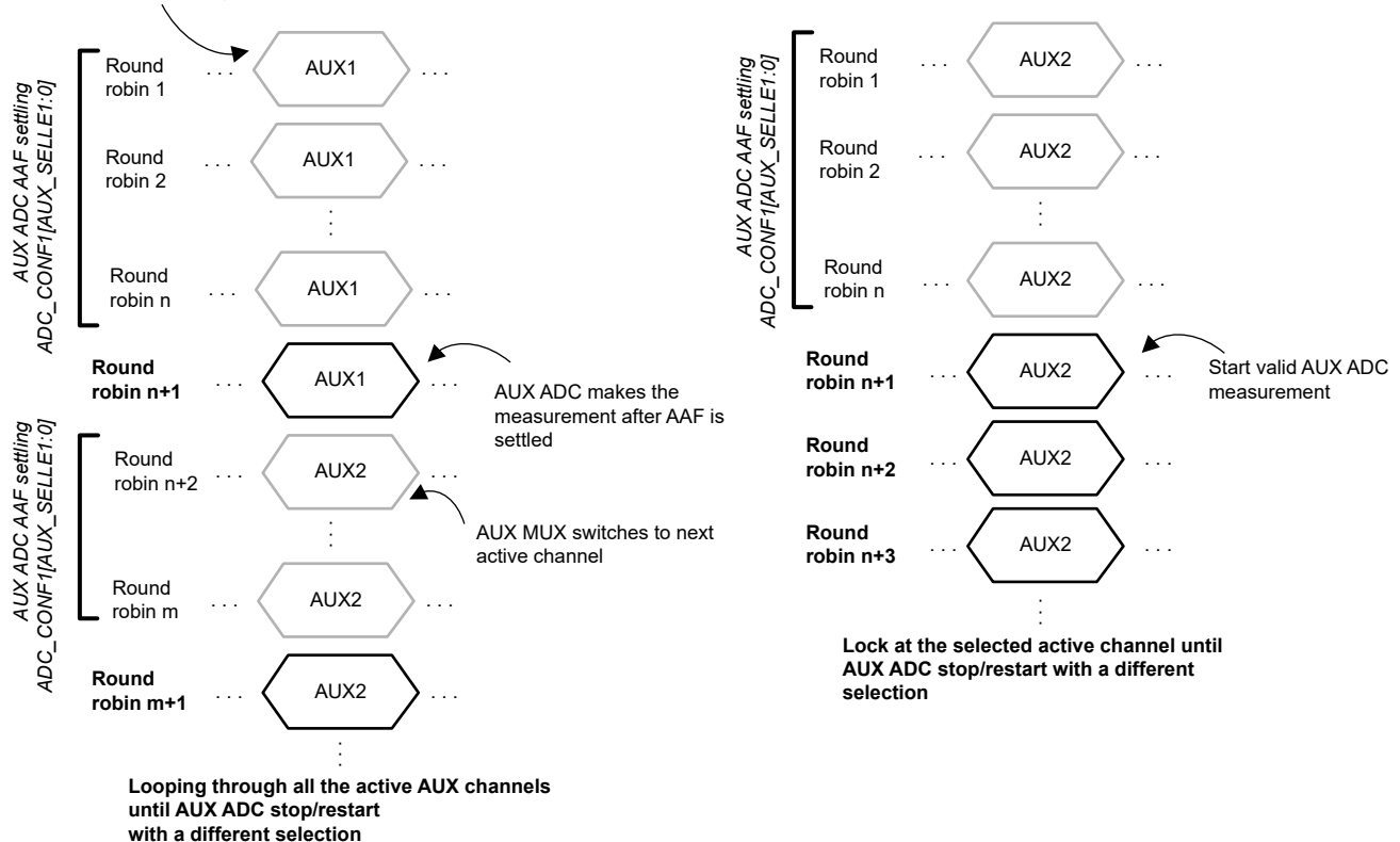
図 8-7. AUX MUX Output Slot with Different [AUX\_IN\_SEL4:0] Setting
