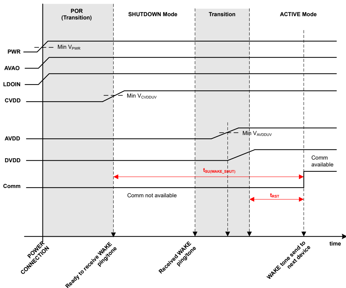
図 8-45. SHUTDOWN to ACTIVE Mode Transition
