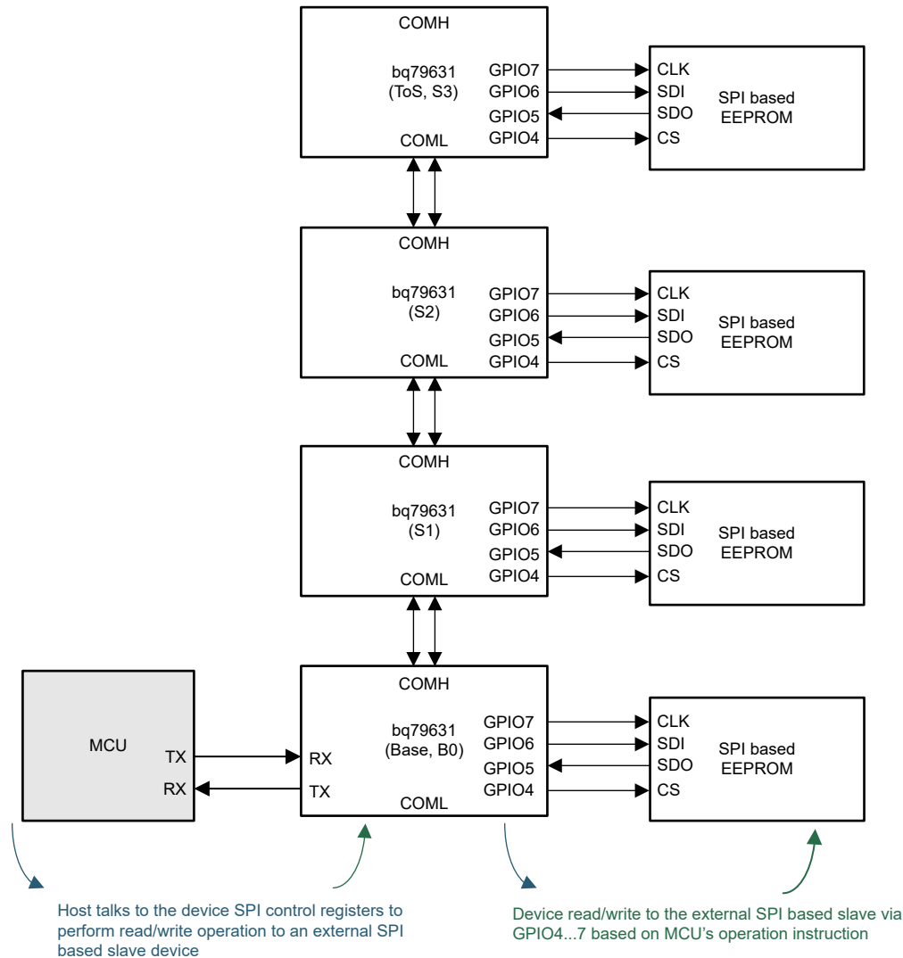
8-32. SPI Master Stack Configuration
