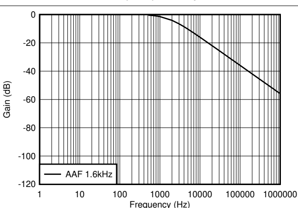
7-4. MAIN ADC Filter
