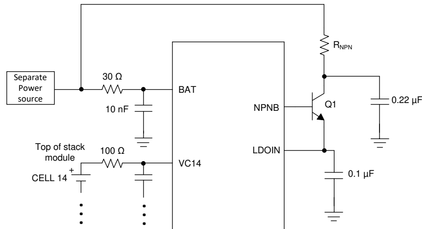
10-4. Separate Power Source to BAT
