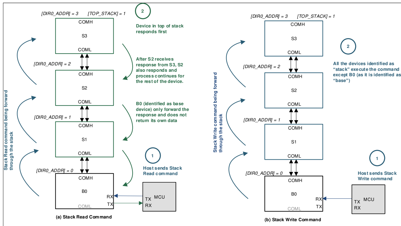
Figure 9-29. Stack Read/Write
