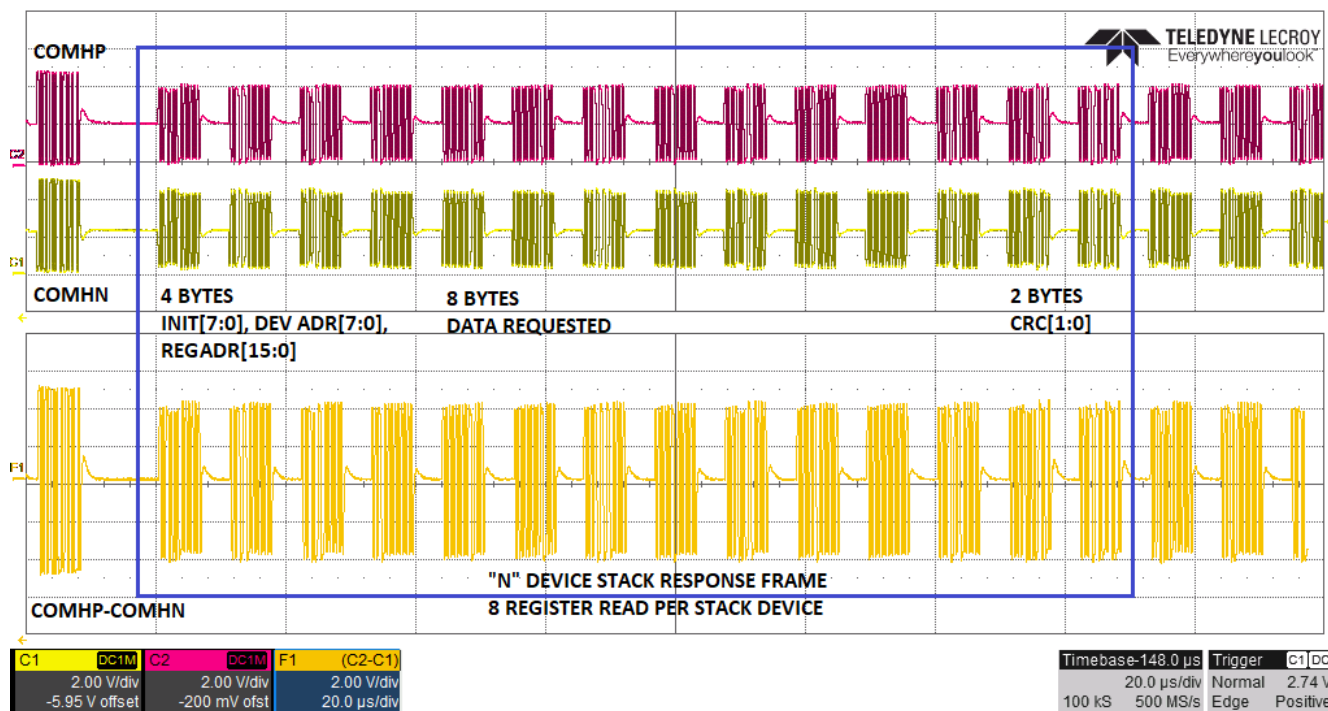
図 9-10. Response Frame for 8 Registers Read from Stack Devices
