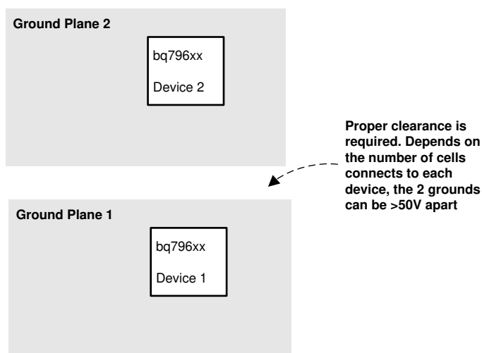
11-2. Separate Ground Planes Per Device on the Same PCB
