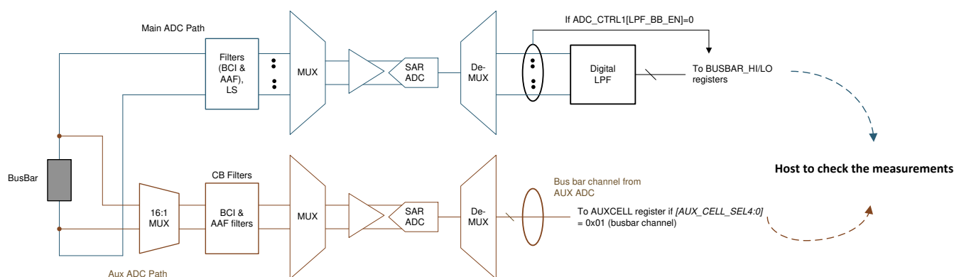
8-54. Bus Bar Through BBP/N Measurement Check
