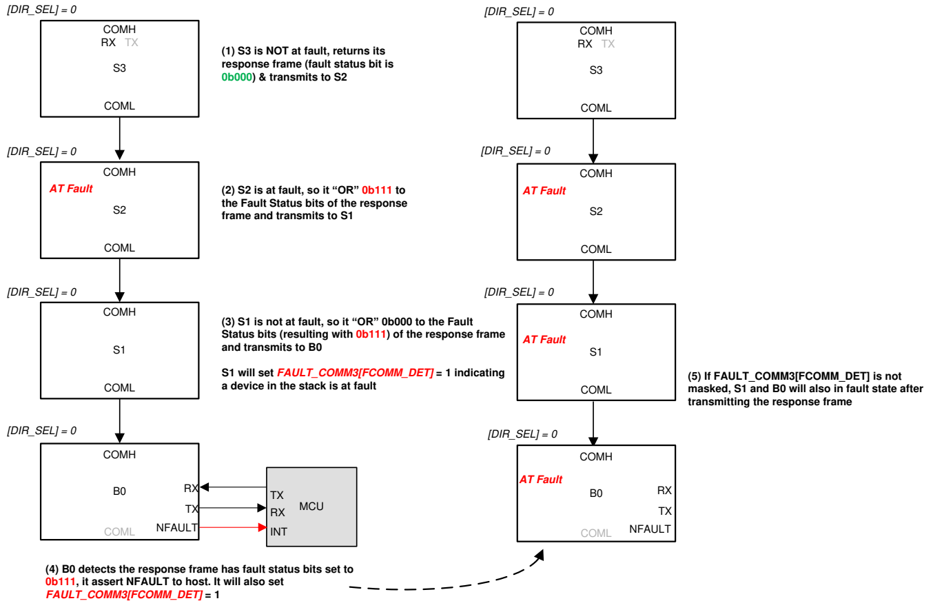
图 8-43. Transfer Fault Status in ACTIVE Mode (Respond to a Single Device Read)
