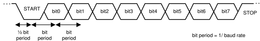
図 8-23. UART Communication to Host
