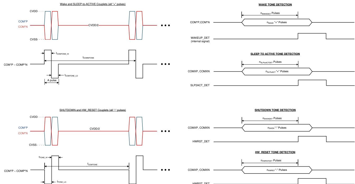
8-63. Communication Tones
