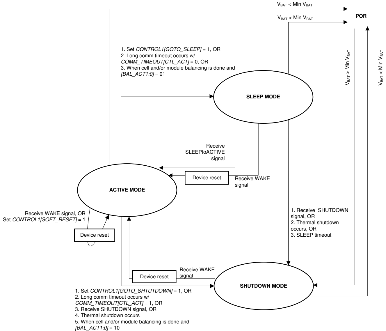
✎ 8-59. Power State Diagram
