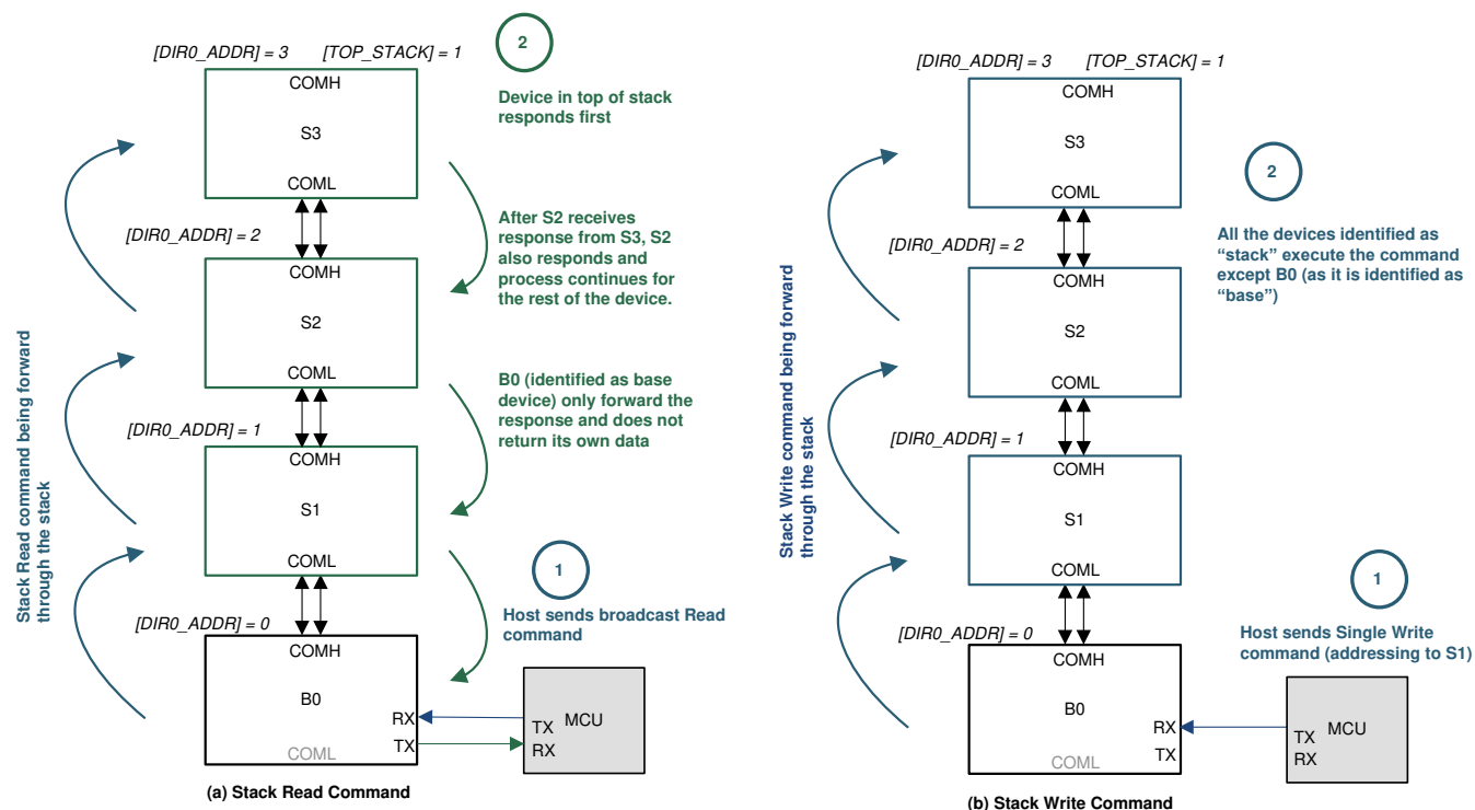
图 8-29. Stack Read/Write
