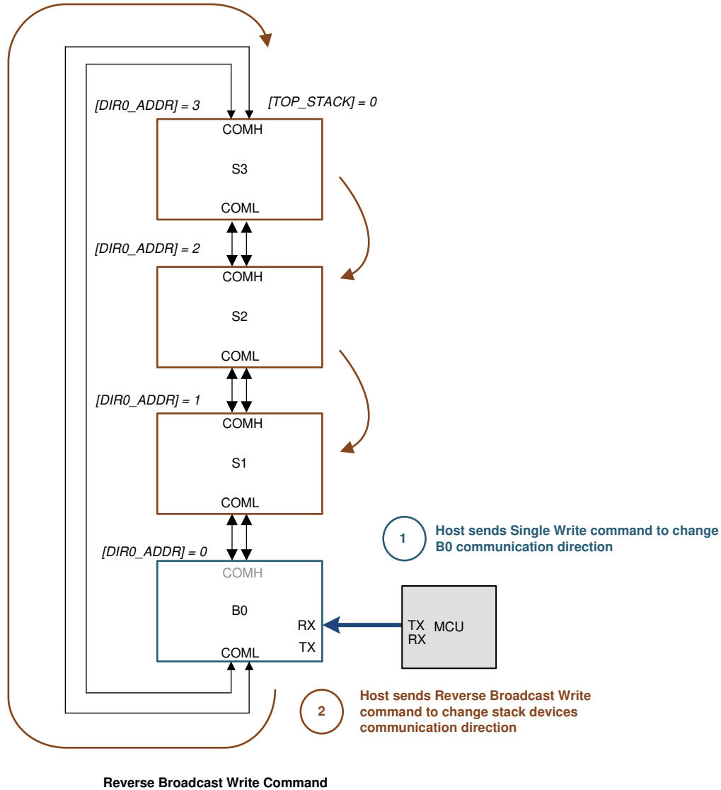
8-31. Broadcast Write Reverse Direction
