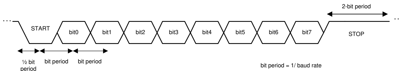
FIG 8-24. UART Response Frame with Two STOP Bits
