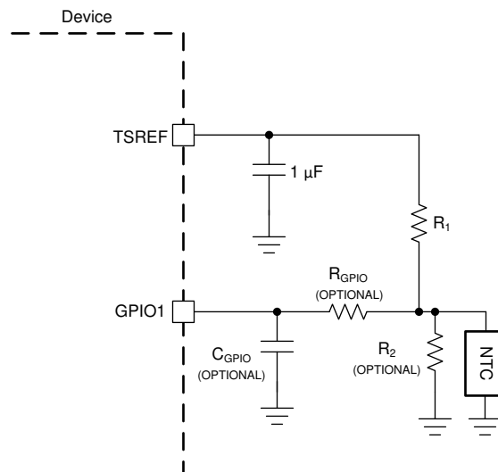
9-5. NTC Connection
