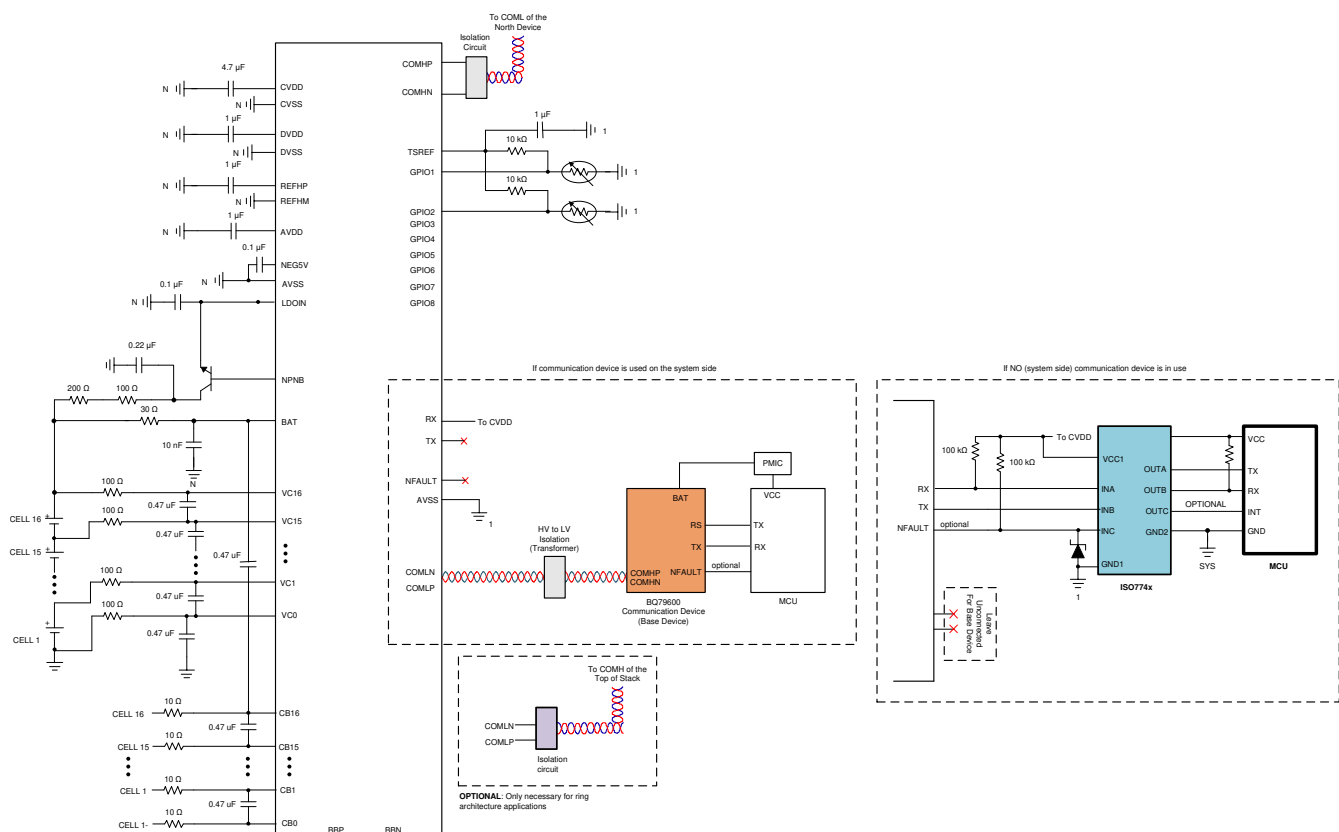
図 9-1. Typical Base Device with Measurement Application Circuit
