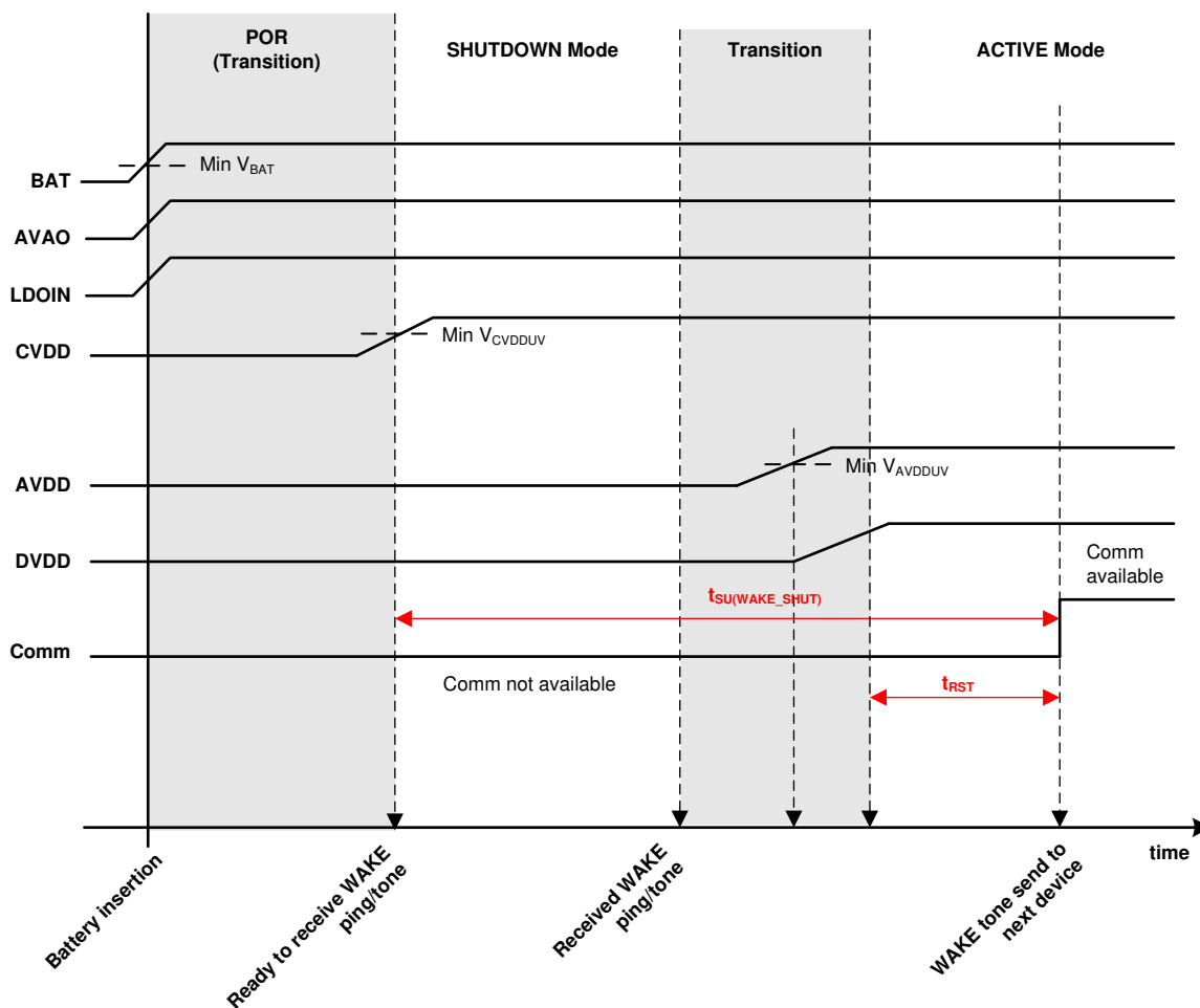
图 8-60. SHUTDOWN to ACTIVE Mode Transition
