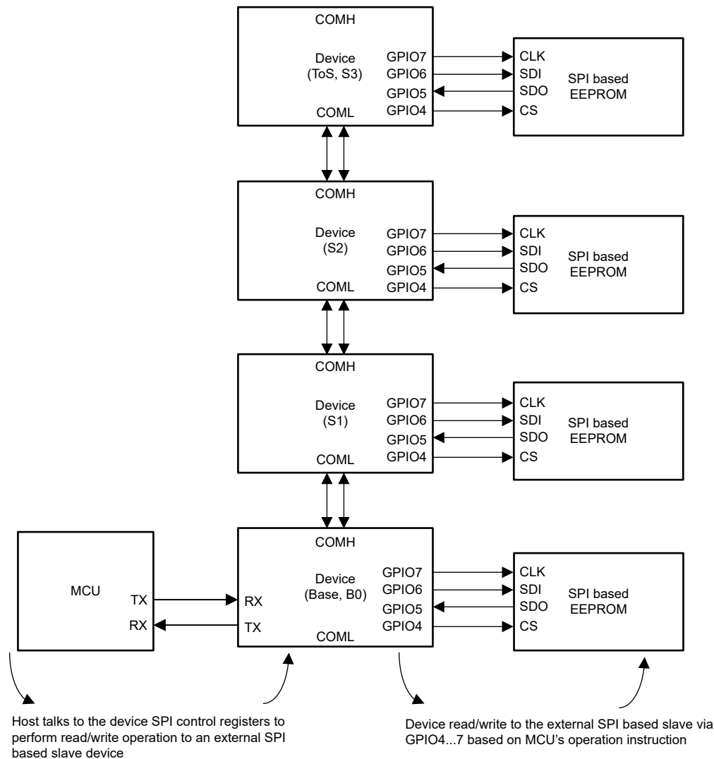
8-39. SPI Controller Stack Configuration
