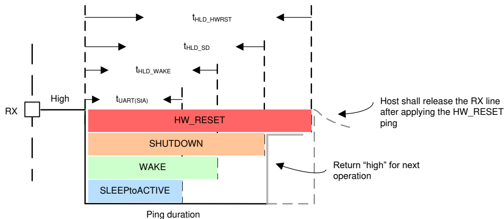
8-62. Communication Pings
