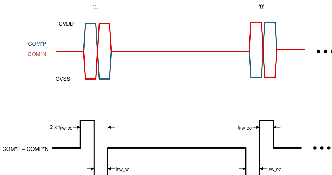
図 8-32. Daisy Chain Bit Definition
