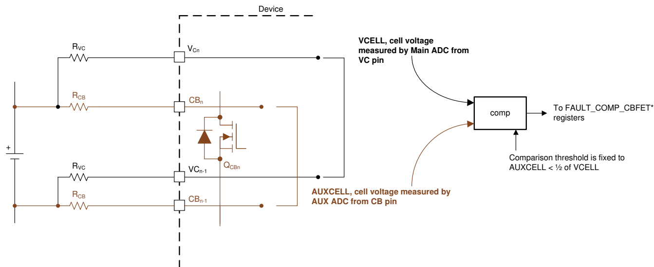
图 8-50. Cell Balancing FET Diagnostic
