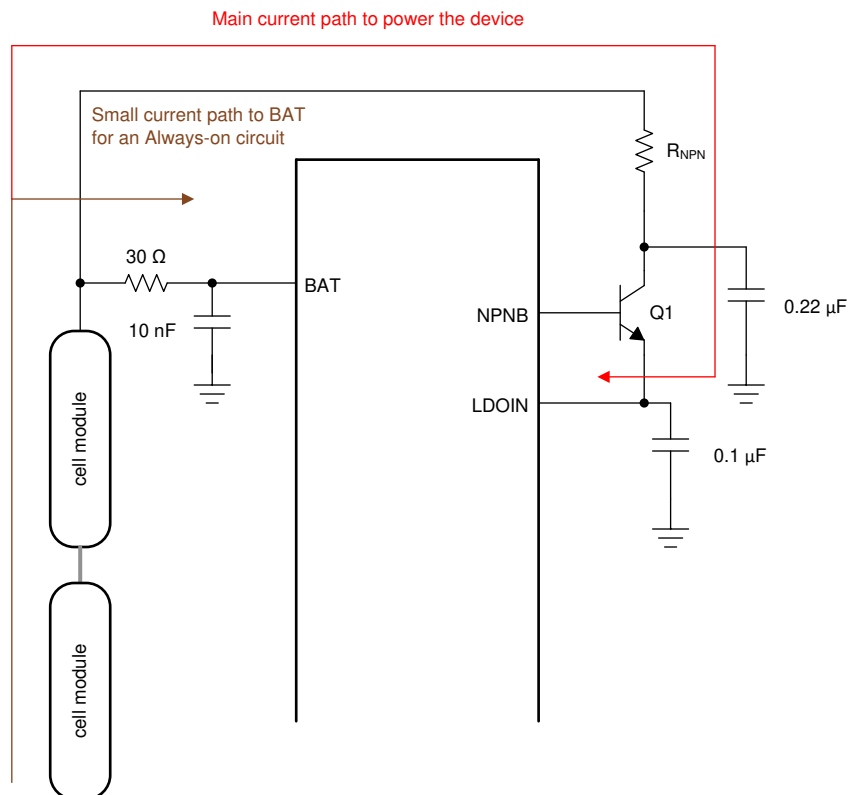
10-2. Device Can Be Powered by Multiple Cell Modules in Stack
