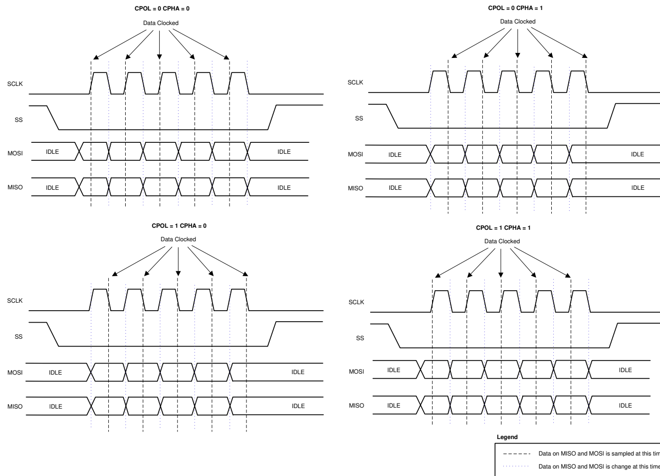
8-40. SPI Controller CPOL and CPHA
