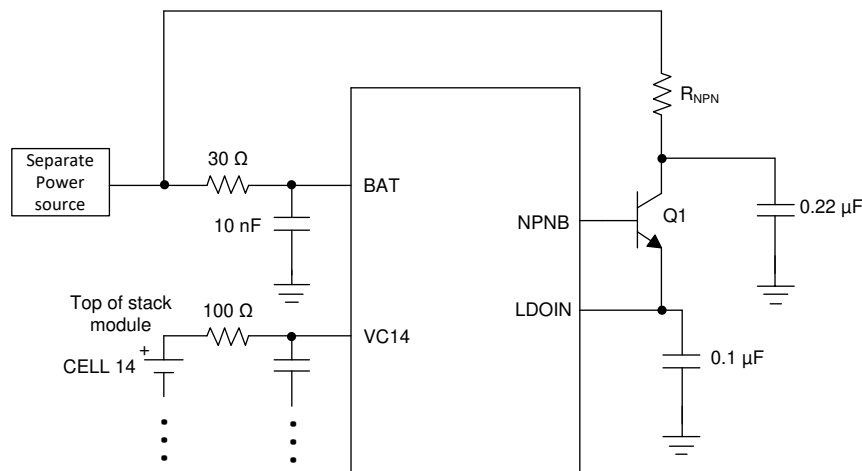
Figure 9-4. Separate Power Source to BAT
