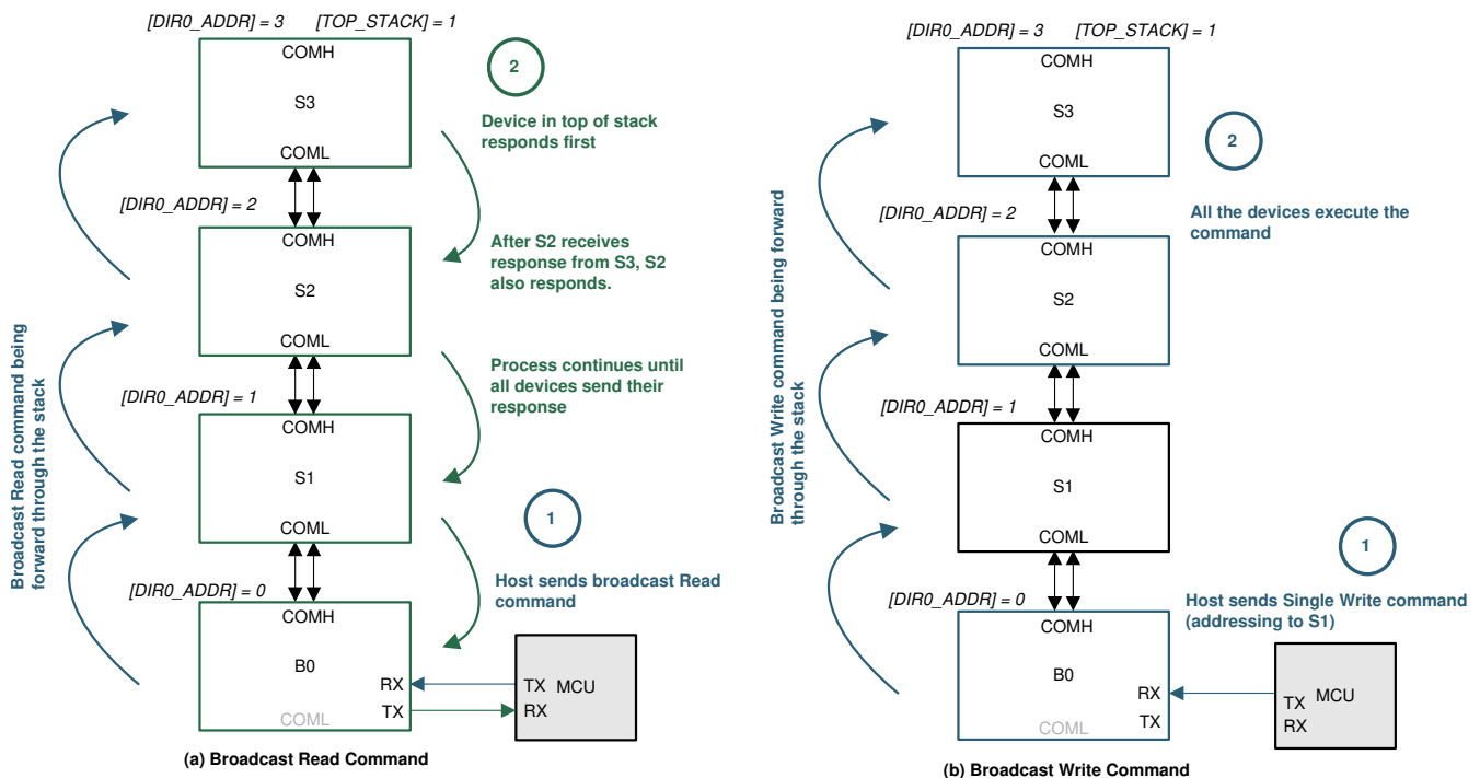
8-30. Broadcast Read/Write
