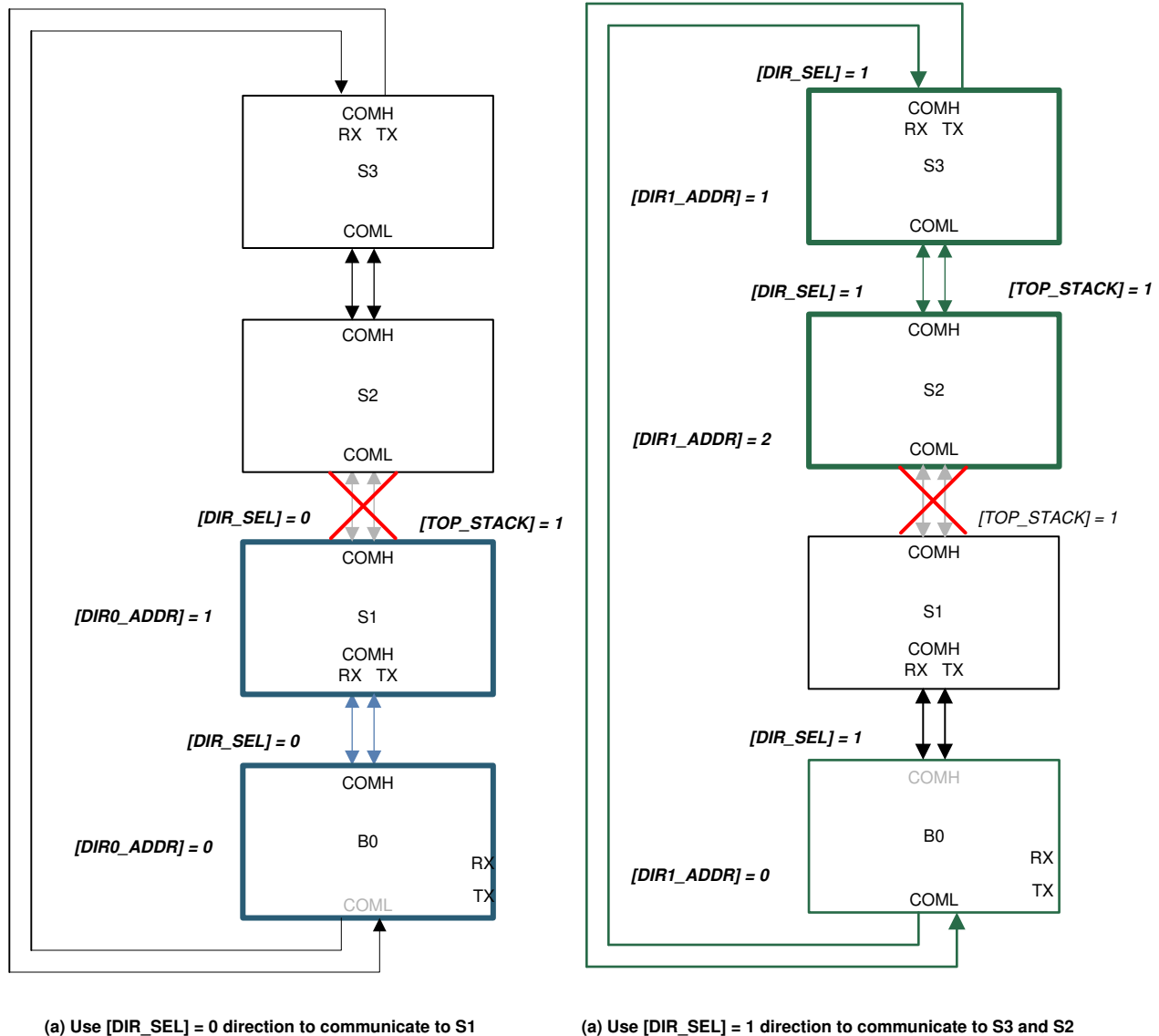
图 8-38. Using Ring Architecture to Access All Devices in a Broken Cable Case
