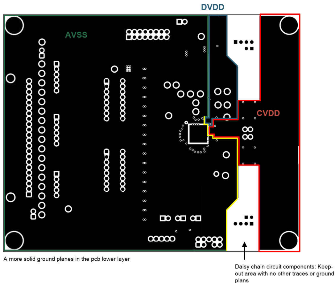
12-5. Second Layer with Solid, Separate Ground Planes
