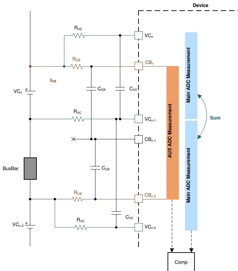
FIG 9-58. Cell Measurement Check with Bus Bar Connected to Individual VC Channel
