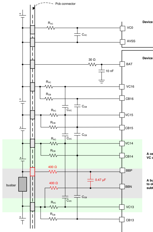
(a) BBP/N connection with bus bar connected in any middle VC channel
