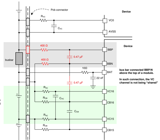
(b) BBP/N connection with bus bar connected above the top of a module
