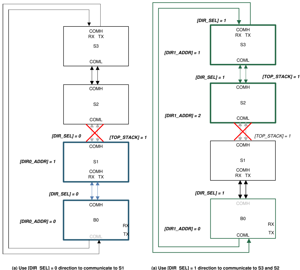
FIG 9-38. Using Ring Architecture to Access All Devices in a Broken Cable Case
