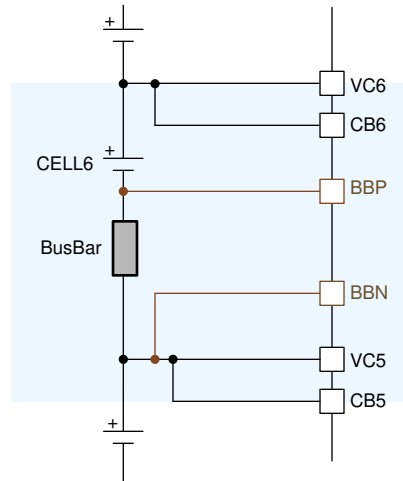
图 9-5. Simplified BBP and BBN Connections
