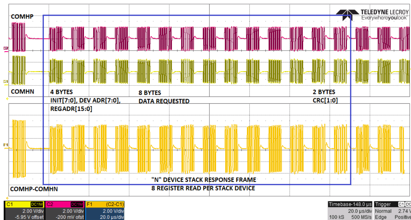
FIG 10-10. Response Frame for 8 Registers Read from Stack Devices
