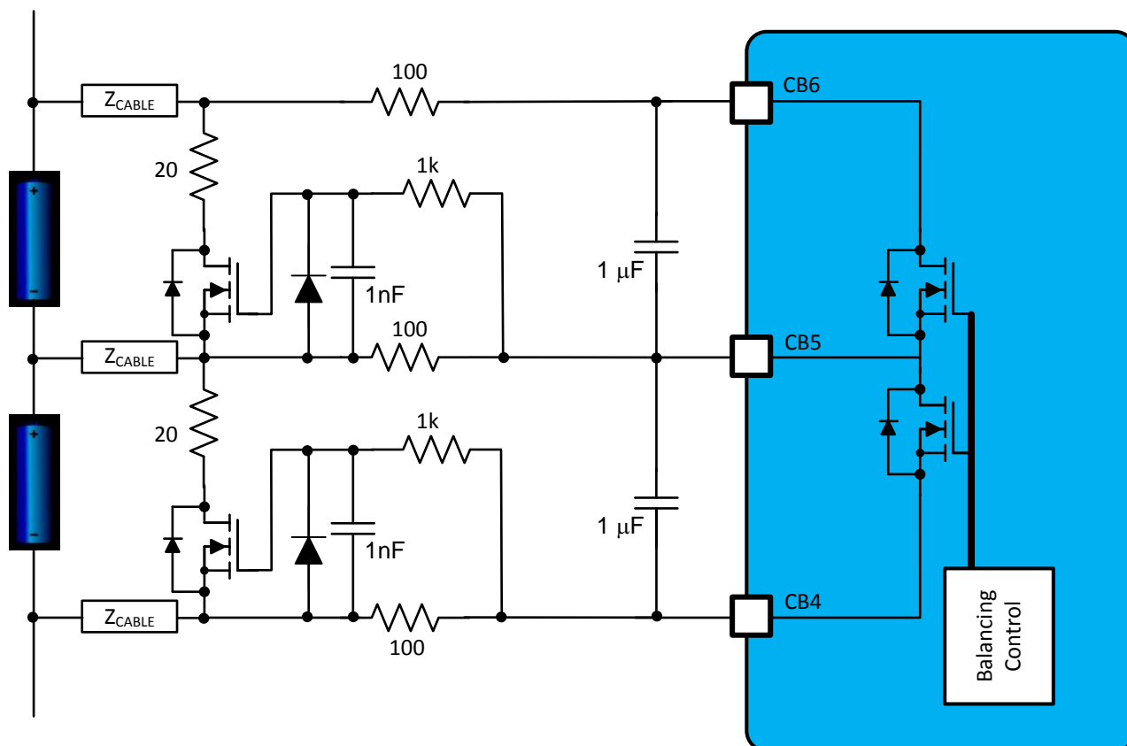
50. Cell Balancing Circuit with External MOSFETs
