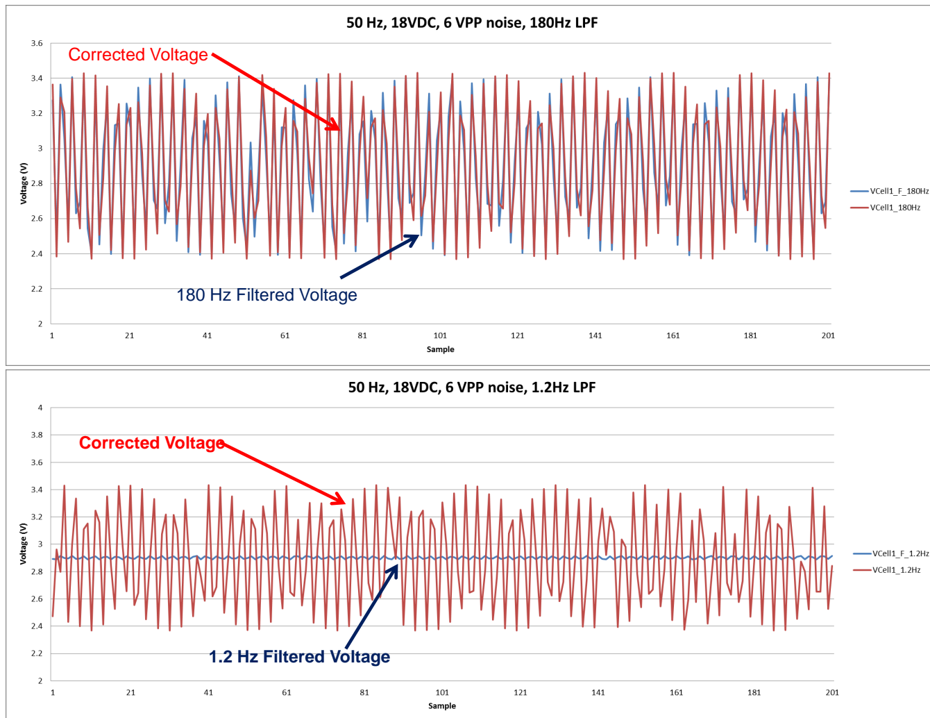
FIG 60. Digital Low Pass Filter Results
