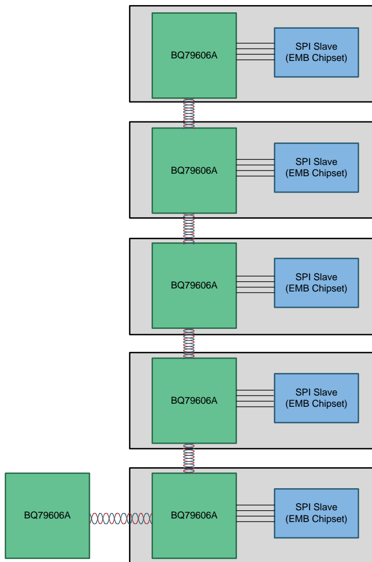
図 34. SPI Master Stack Configuration
