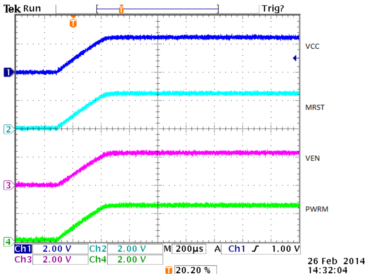
Figure 10. VCC, MRST, VEN, and PWRM Upon Power Up
