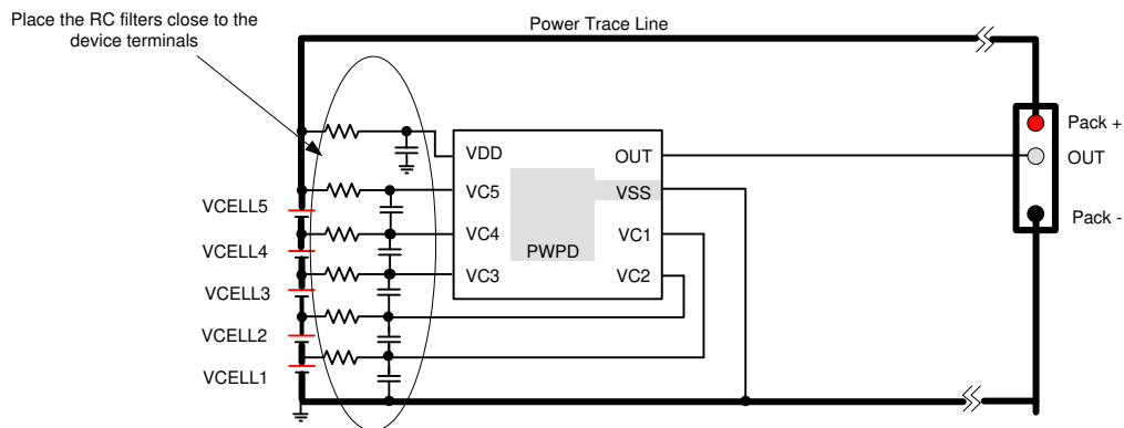
✎ 11-1. Example Layout
