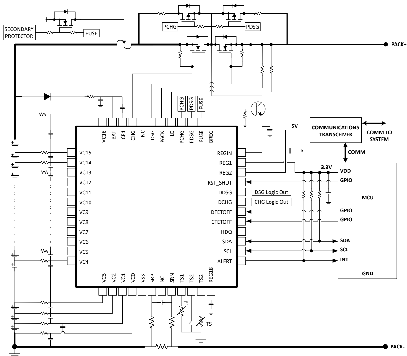
図 16-1. BQ76952 16-Series Cell Typical Implementation (Simplified Schematic)
