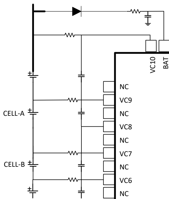
FIG 10-2. Terminating an Unused Cell Input Pin
