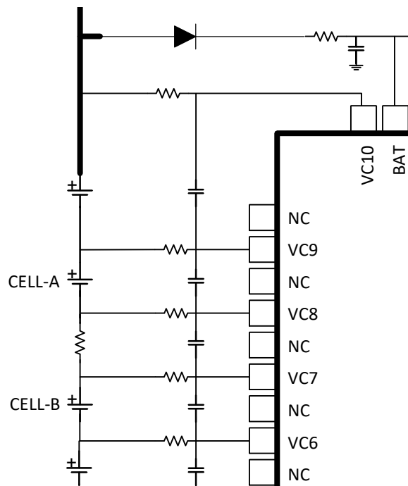
FIG 10-1. Using Cell Input Pins for Interconnect Measurement
