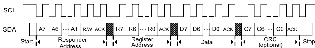
14-1. I 2 C Write
