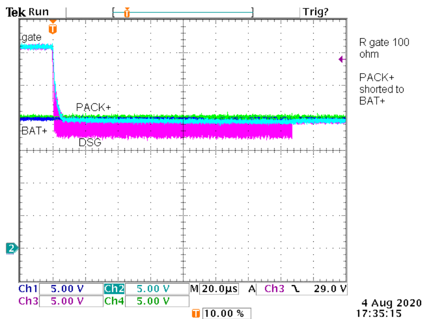
8-11. A Fast Turn-Off Case with a 100- \Omega Series Gate Resistor
