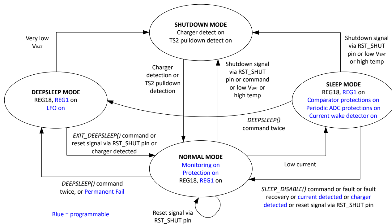
7-5. Device Functional Modes
