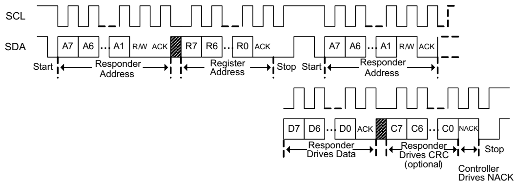
図 7-8. I 2 C Read Without Repeated Start
