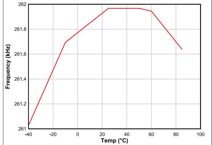
Figure 6-12. Low Frequency Oscillator (LFO) Accuracy vs Temperature
