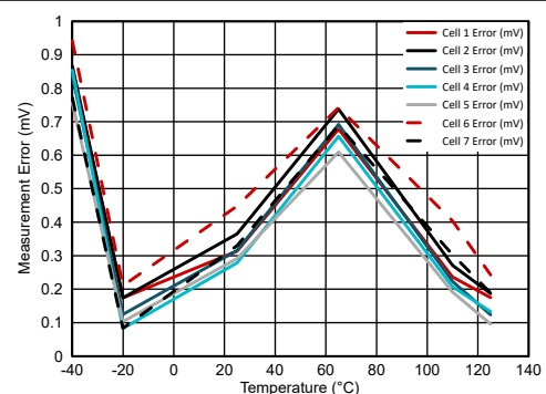
図 6-5. Cell Voltage Measurement Error vs. Temperature with Cell Voltage = 1.5 V
