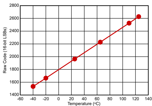
図 6-16. Internal Temperature Measurement Raw Codes vs. Temperature
