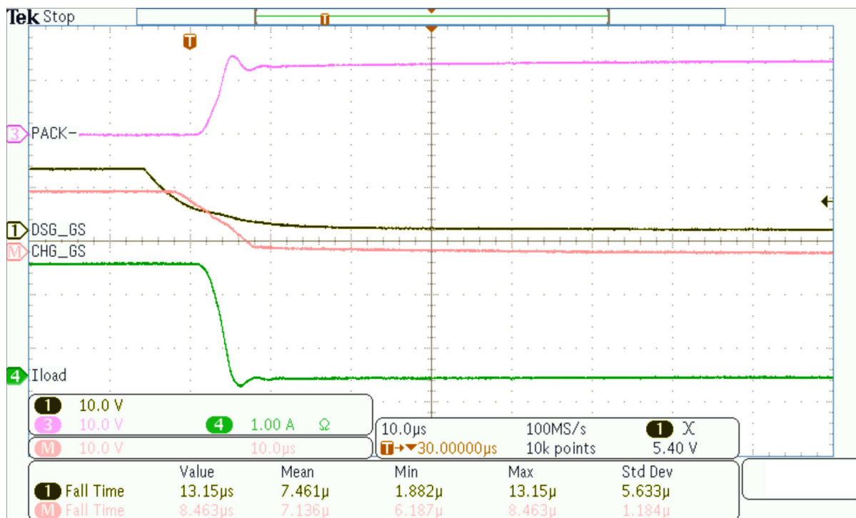
図 8-6. Moderate Speed FET Turn-Off, Using a 1.35-k \Omega Series Gate Resistor, and a 2A Load between \text{PACK+} and \text{PACK-} .
