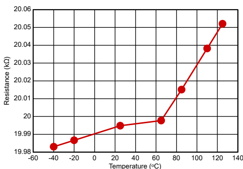
図 6-18. Thermistor Pullup Resistance vs. Temperature
