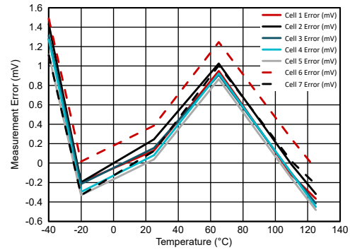
図 6-9. Cell Voltage Measurement Error vs. Temperature with Cell Voltage = 3.5 V
