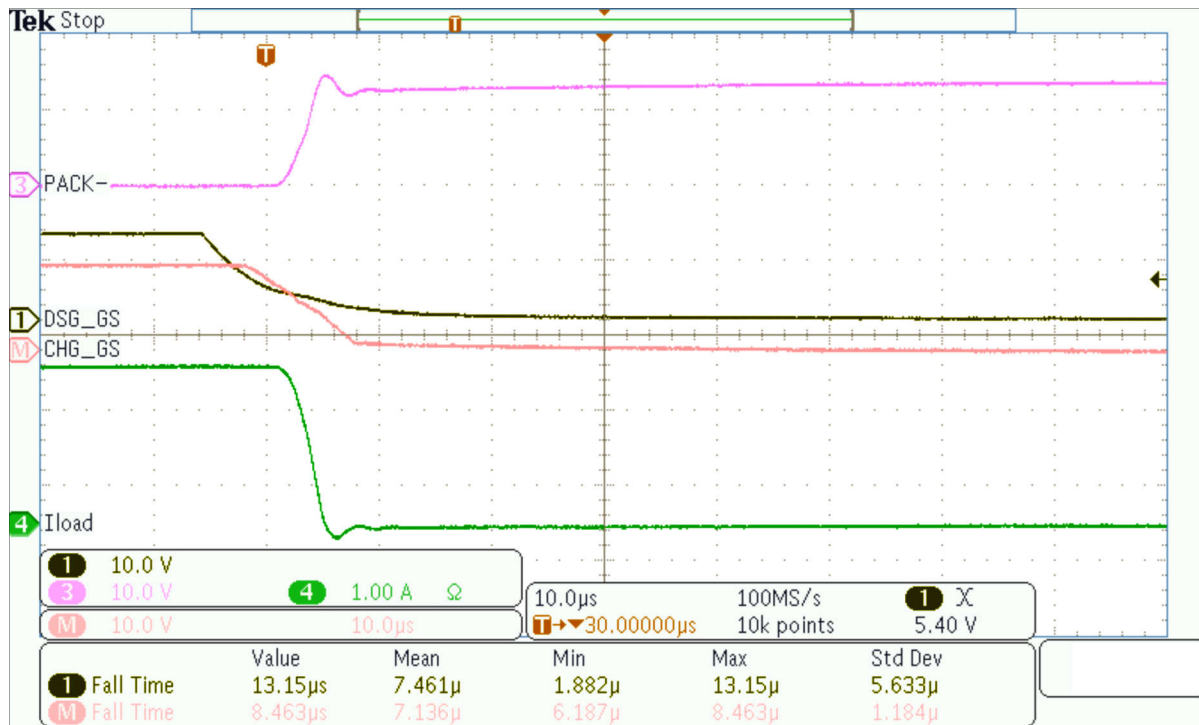
図 8-6. Moderate Speed FET Turn-Off, Using a 1.35-k \Omega Series Gate Resistor, and a 2A Load between PACK+ and PACK- .
