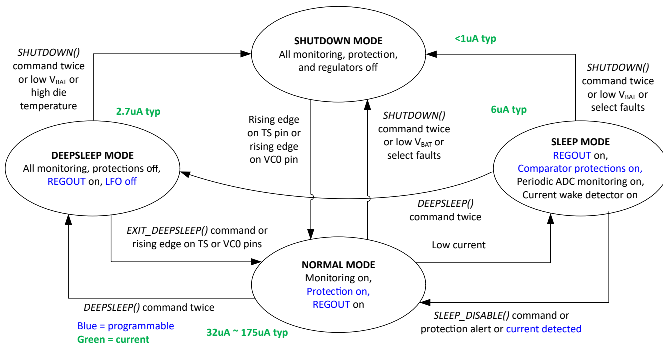
图 7-5. BQ76907 Operational Power Modes
