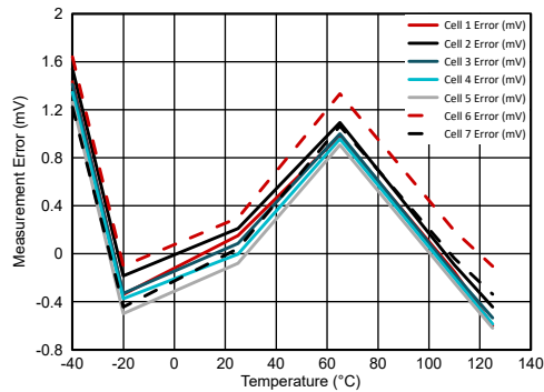
図 6-10. Cell Voltage Measurement Error vs. Temperature with Cell Voltage = 4.0 V
