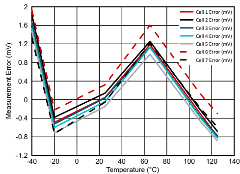
図 6-12. Cell Voltage Measurement Error vs. Temperature with Cell Voltage = 5.0 V
