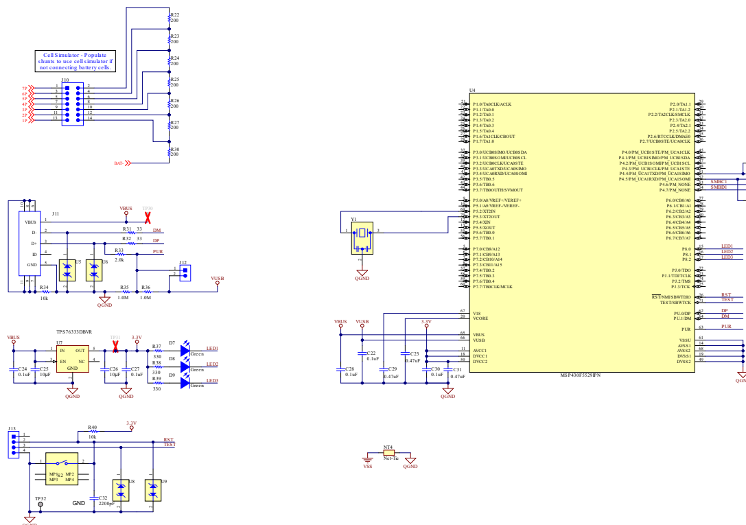
図 8-3. BQ76907 7-Series Cell Schematic Diagram—Additional Circuitry
