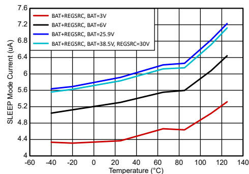
図 6-27. Supply Current in SLEEP Mode vs. Temperature
