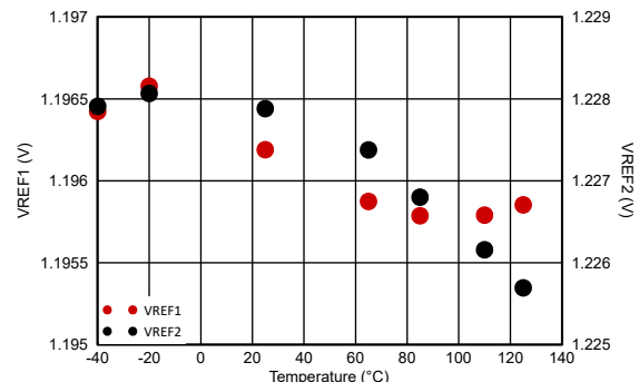
図 6-15. Internal Voltage References vs. Temperature (VREF1 and VREF2)
