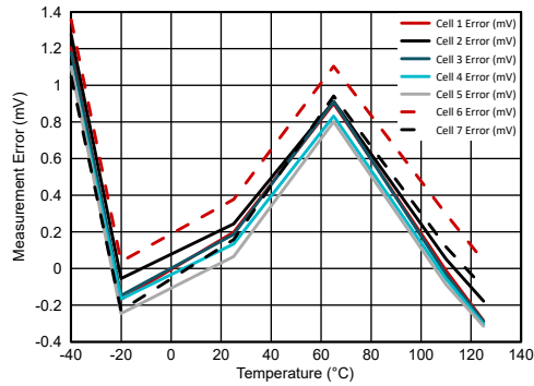
図 6-8. Cell Voltage Measurement Error vs. Temperature with Cell Voltage = 3.0 V
