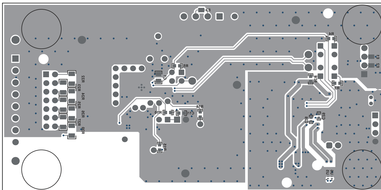
図 10-2. BQ76907 Two-Layer Board Layout—Bottom Layer
