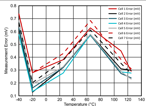
図 6-4. Cell Voltage Measurement Error vs. Temperature with Cell Voltage = 1.0 V
