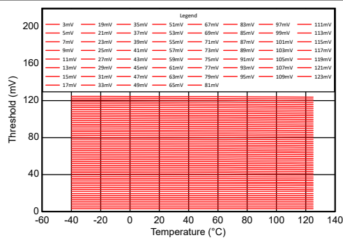
図 6-21. Overcurrent in Charge Protection (OCC) Threshold vs. Temperature
