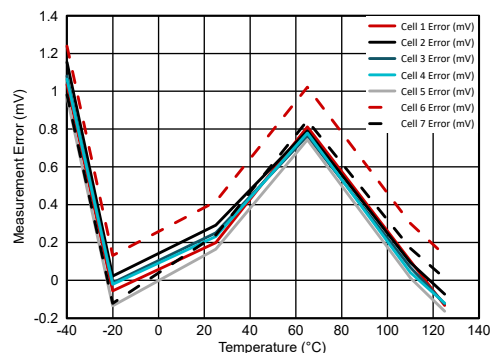
図 6-7. Cell Voltage Measurement Error vs. Temperature with Cell Voltage = 2.5 V
