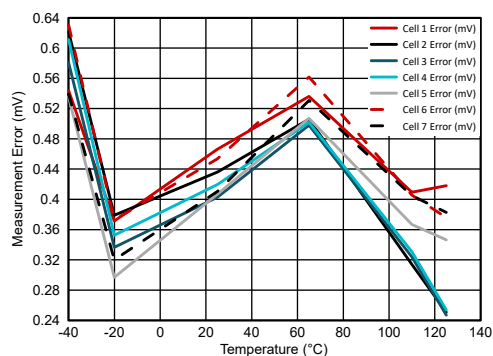
図 6-3. Cell Voltage Measurement Error vs. Temperature with Cell Voltage = 0.5 V
