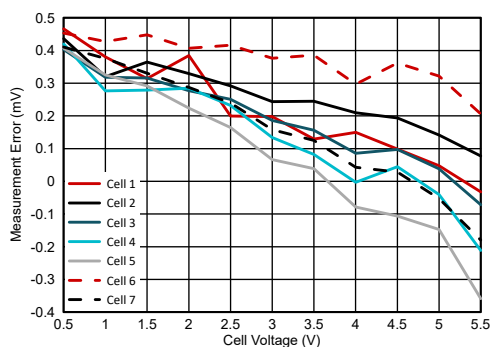
図 6-2. Cell Voltage Measurement Error at 25°C Across Input Range
