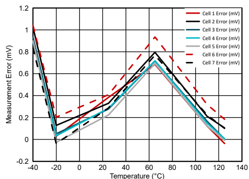
図 6-6. Cell Voltage Measurement Error vs. Temperature with Cell Voltage = 2.0 V
