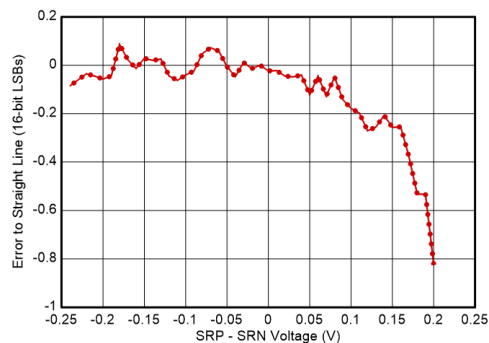
図 6-14. Current Linearity Error vs. Sense Resistor Voltage
