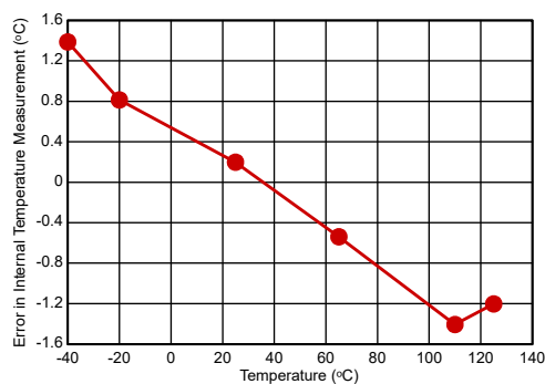
図 6-17. Internal Temperature Measurement Error vs. Temperature
