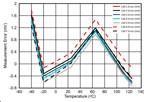
図 6-11. Cell Voltage Measurement Error vs. Temperature with Cell Voltage = 4.5 V
