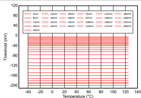
図 6-20. Overcurrent in Discharge Protection 1 (OCD1) Threshold vs. Temperature
