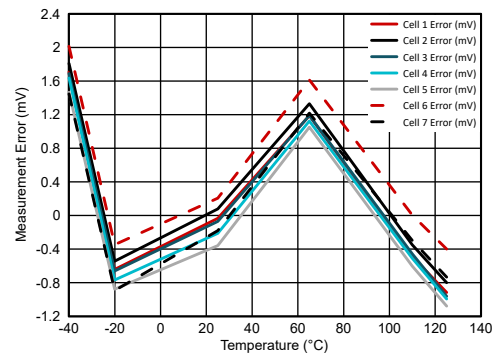
図 6-13. Cell Voltage Measurement Error vs. Temperature with Cell Voltage = 5.5 V
