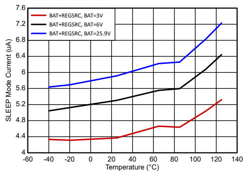
Figure 6-27. Supply Current in SLEEP Mode vs. Temperature
