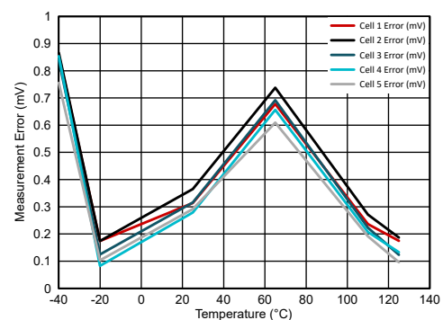
Figure 6-5. Cell Voltage Measurement Error vs. Temperature with Cell Voltage = 1.5 V
