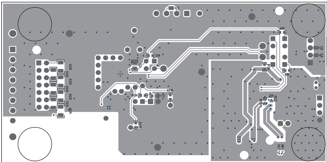
図 8-10. BQ76905 Two-Layer Board Layout–Bottom Layer
