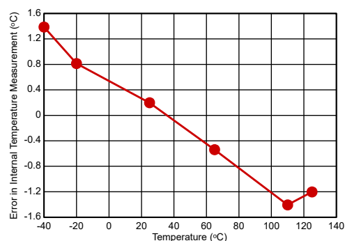
図 6-17. Internal Temperature Measurement Error vs. Temperature
