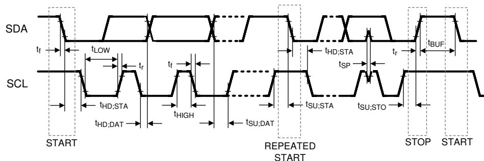
図 6-1. I 2 C Communications Interface Timing
