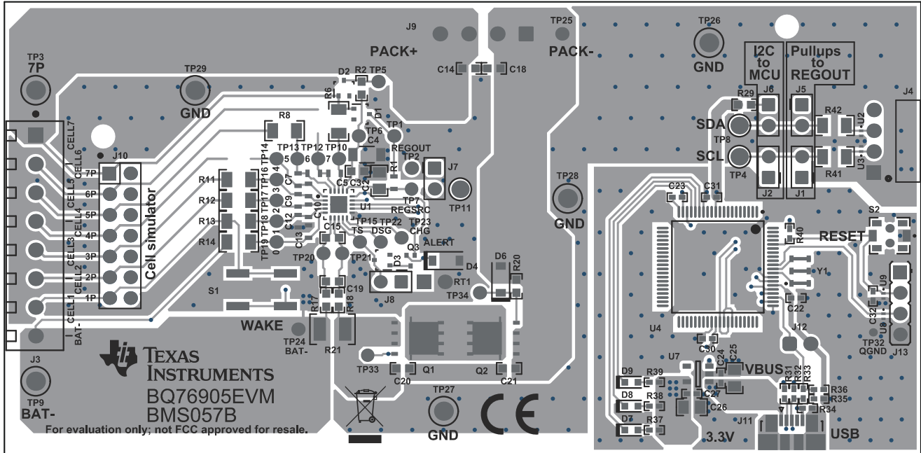
図 8-9. BQ76905 Two-Layer Board Layout–Top Layer
