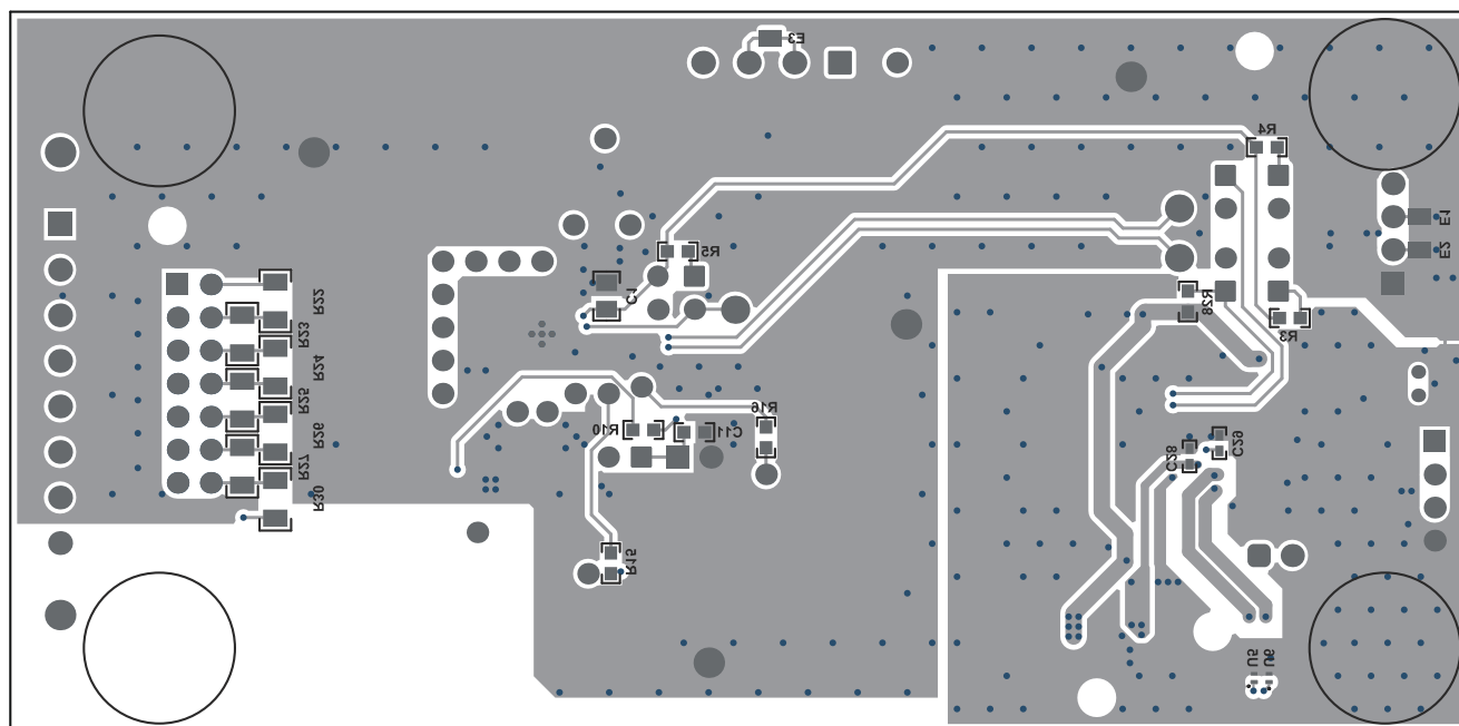
図 8-10. BQ76905 Two-Layer Board Layout–Bottom Layer
