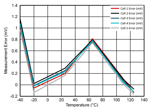
Figure 6-7. Cell Voltage Measurement Error vs. Temperature with Cell Voltage = 2.5 V
