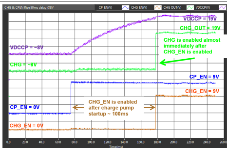
FIG 12. CHG_EN Switched On After Charger Pump Turns On and is Stable
