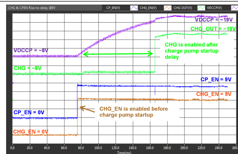
FIG 13. CHG_EN Enabled Before Charge Pump is Turned On
