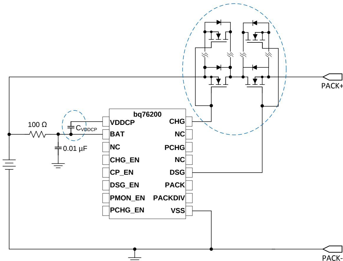
FIG 8. Scale C_{VDDCP} to Support Multiple FETs in Parallel (Partial Schematic Shown)
