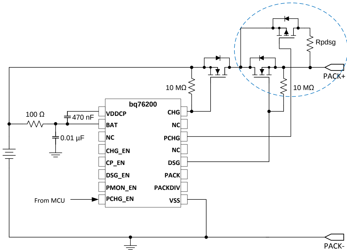
FIG 10. P-Channel FET in Parallel with DSG FET for Pre-Discharging (Partial Schematic Shown)
