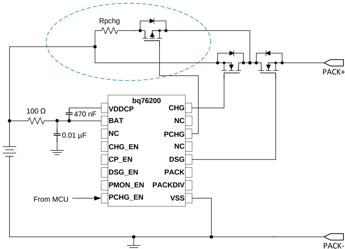
FIG 9. P-Channel FET in Parallel With CHG FET for Pre-Charging (Partial Schematic Shown)
