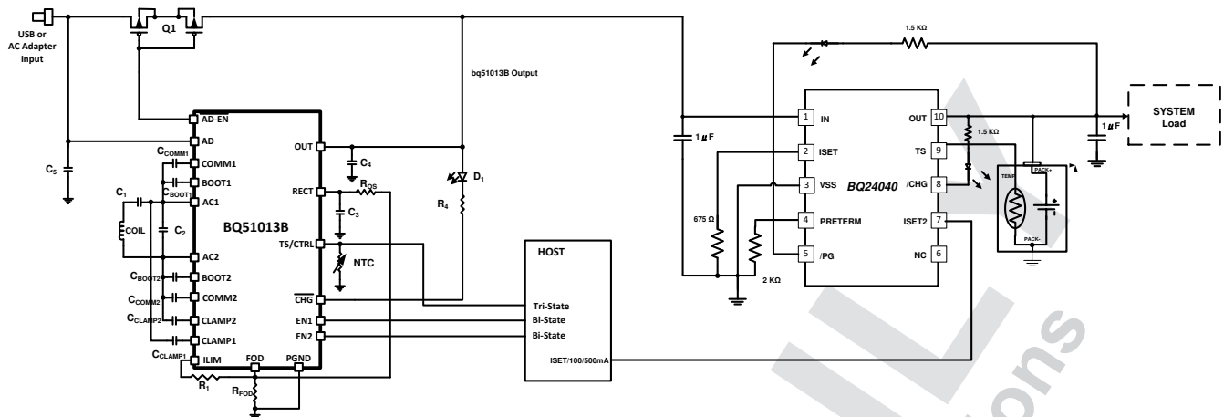
FIG 9-11. BQ51013B Used as a Wireless Power Supply With Adapter Multiplexing for a Linear Charger
