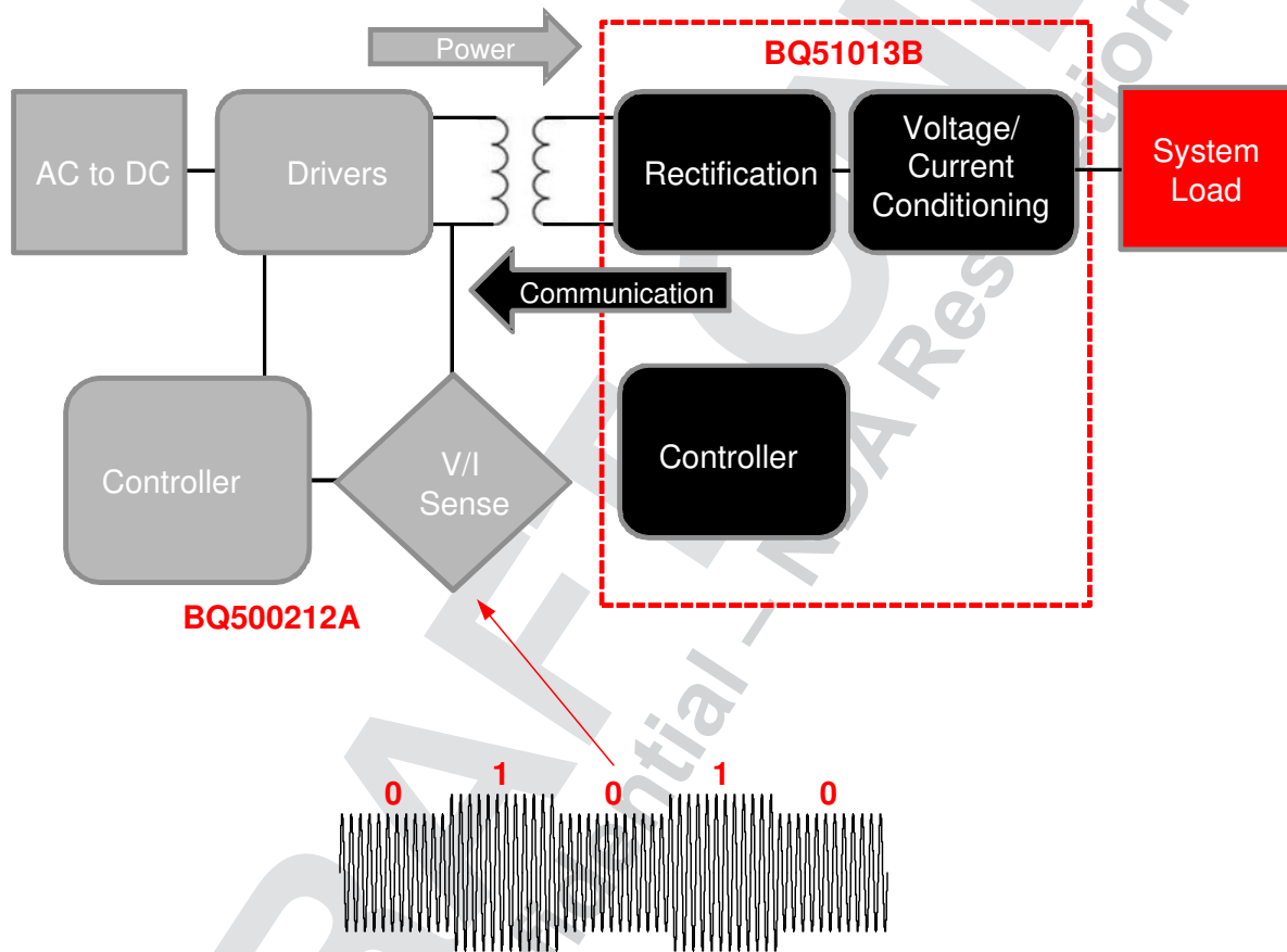
8-6. TX Coil Voltage/Current
