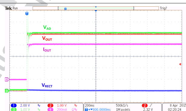
☒ 9-10. AD Power Start-Up With No Transmitter (EN1 = EN2 = LOW)
