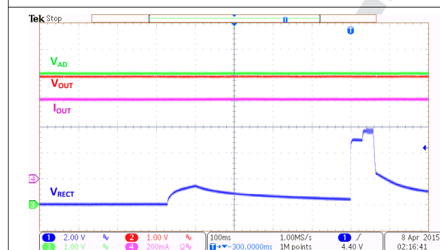
☒ 9-9. Wireless Power Start-Up With V_{\text{AD}} = 5 \text{ V} (EN1 = EN2 = LOW)
