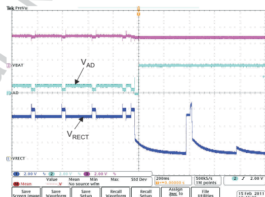
7-16. On-the-Go Enabled ( V_{OTG} = 3.5 \text{ V} ) (3)
