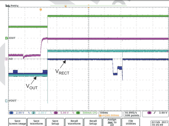
7-14. Adapter Insertion ( V_{AD} = 10 \text{ V} )
