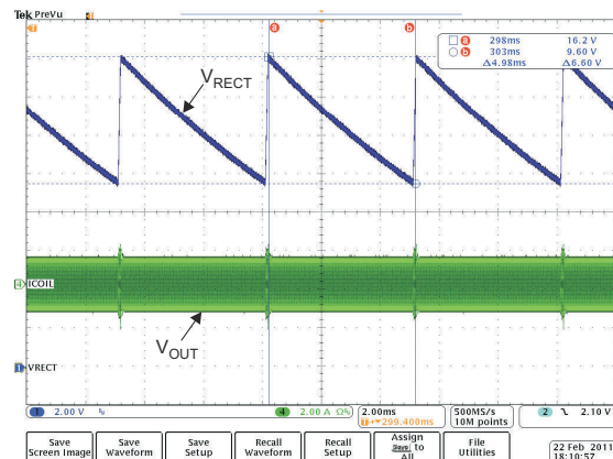
7-12. Rectifier Overvoltage Clamp ( f_{op} = 110 \text{ kHz} )
