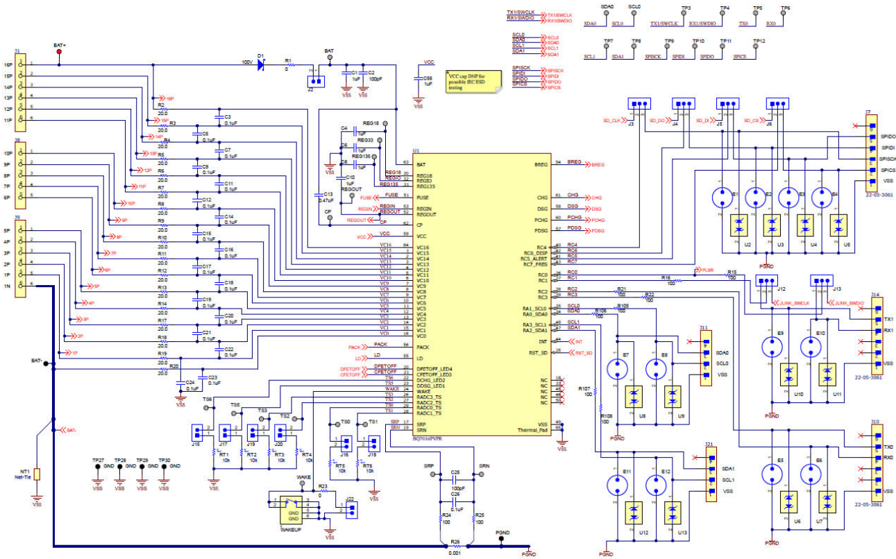
図 8-1. Typical Applications
