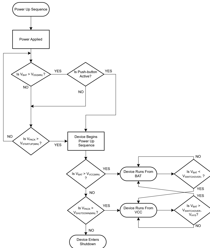
7-1. Power-Up Sequence
