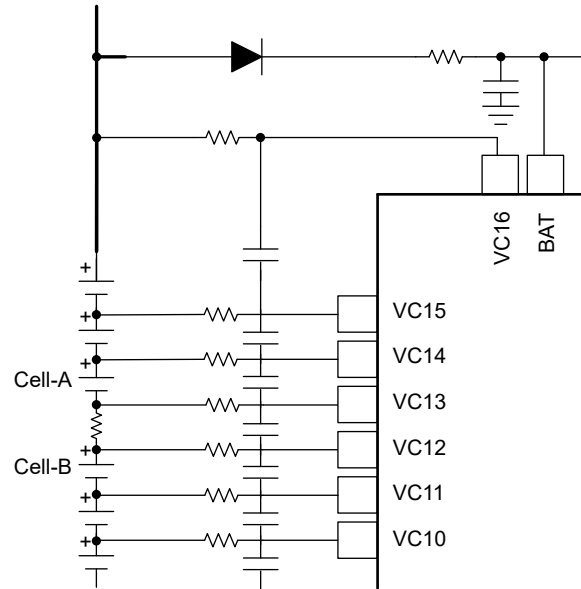
図 7-3. Using Cell Input Pins for Interconnect Measurement
