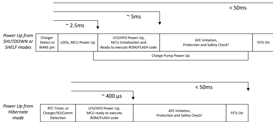
図 7-2. Device Wake-Up Timing
