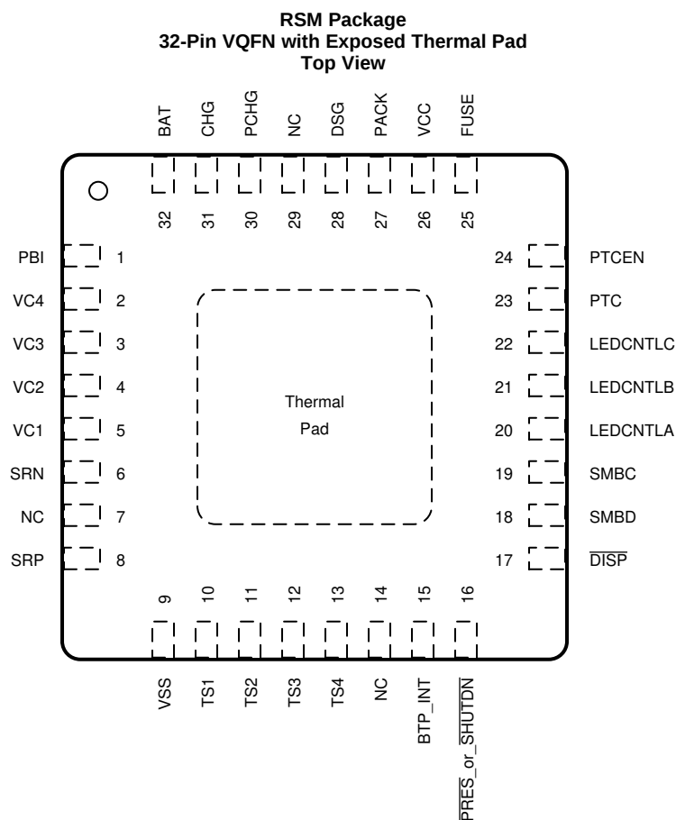
Pin Functions
