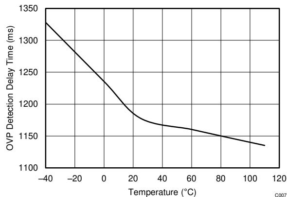
図 6-7. OVP Detection Delay Time Versus Temperature
