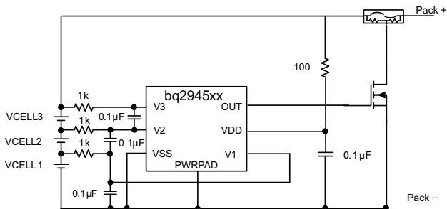
FIG 9-4. 3-Series Cell Configuration with Fixed Delay
