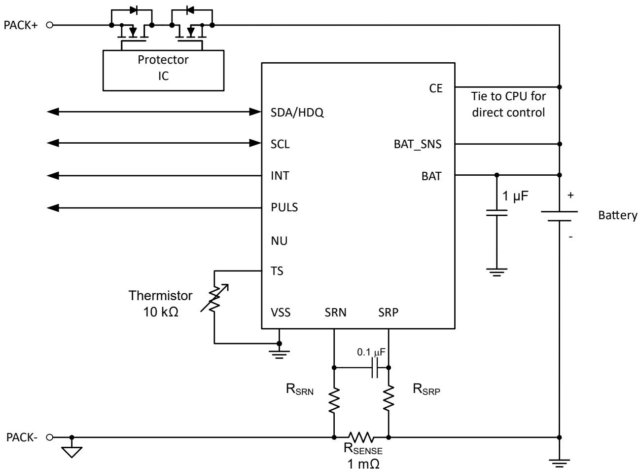
FIG 9-1. BQ27Z561-R1 Typical Implementation with Low-side Current Sensing
