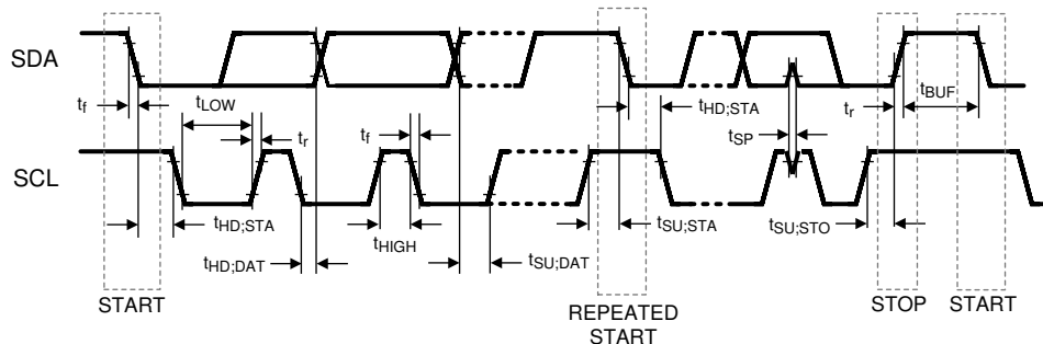
7-1. I²C Timing
