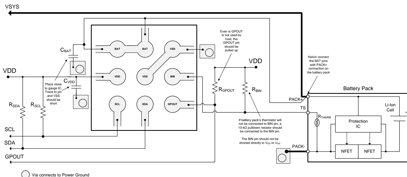
Figure 13. Layout Example
