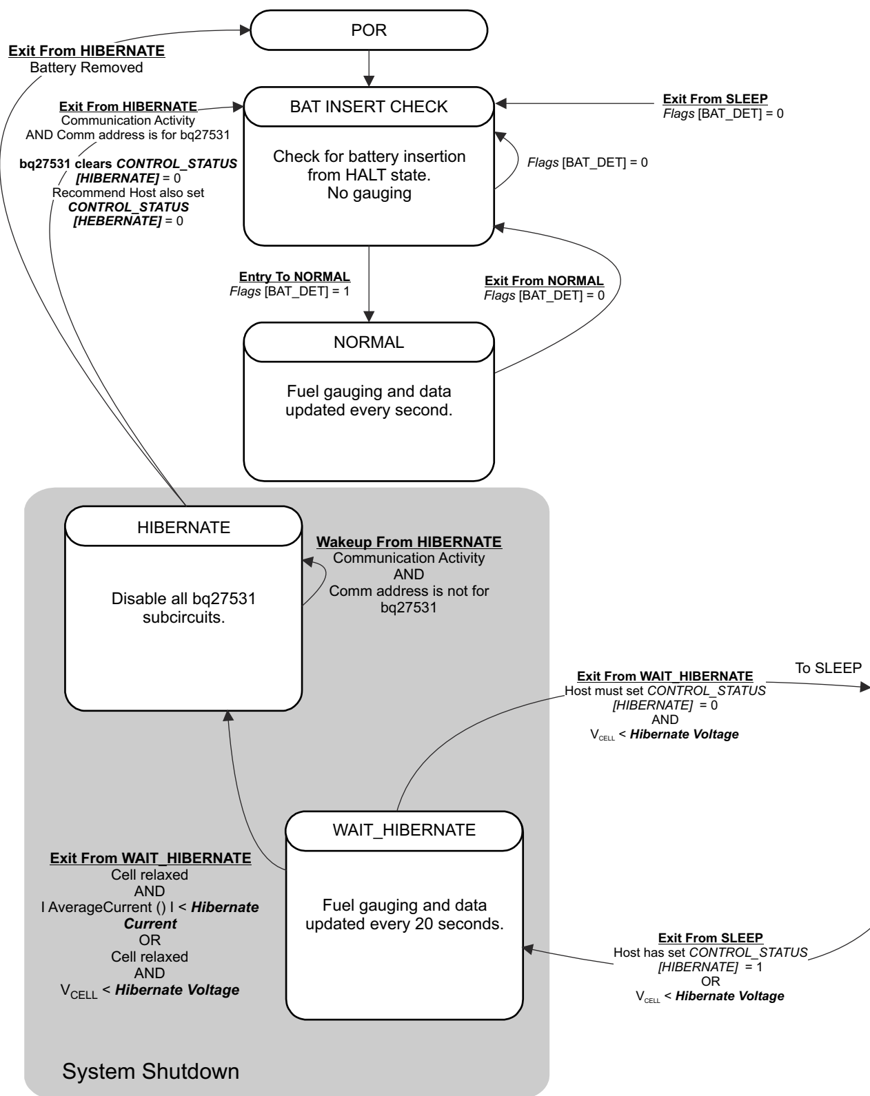
8-2. Power Mode Diagram—System Shutdown
