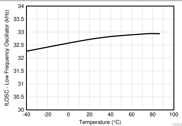
7-4. Low-Frequency Oscillator Frequency vs. Temperature
