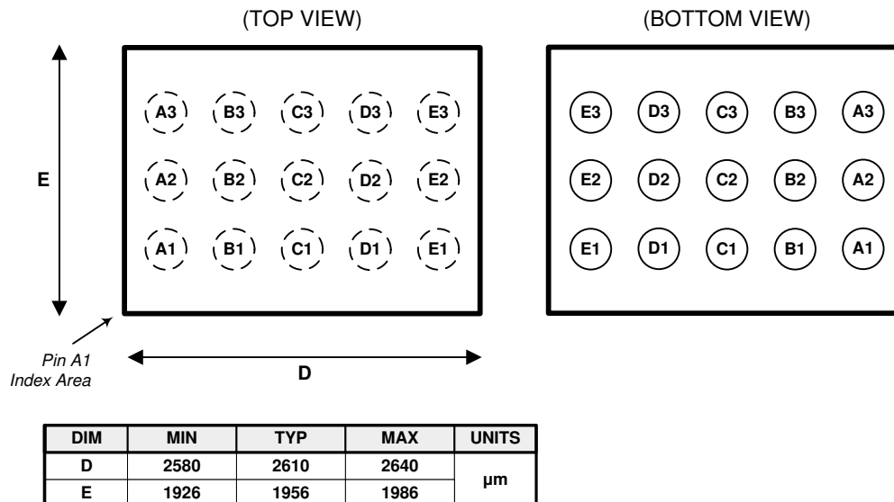
6-1. YZF Package 15-Pin DSBGA
