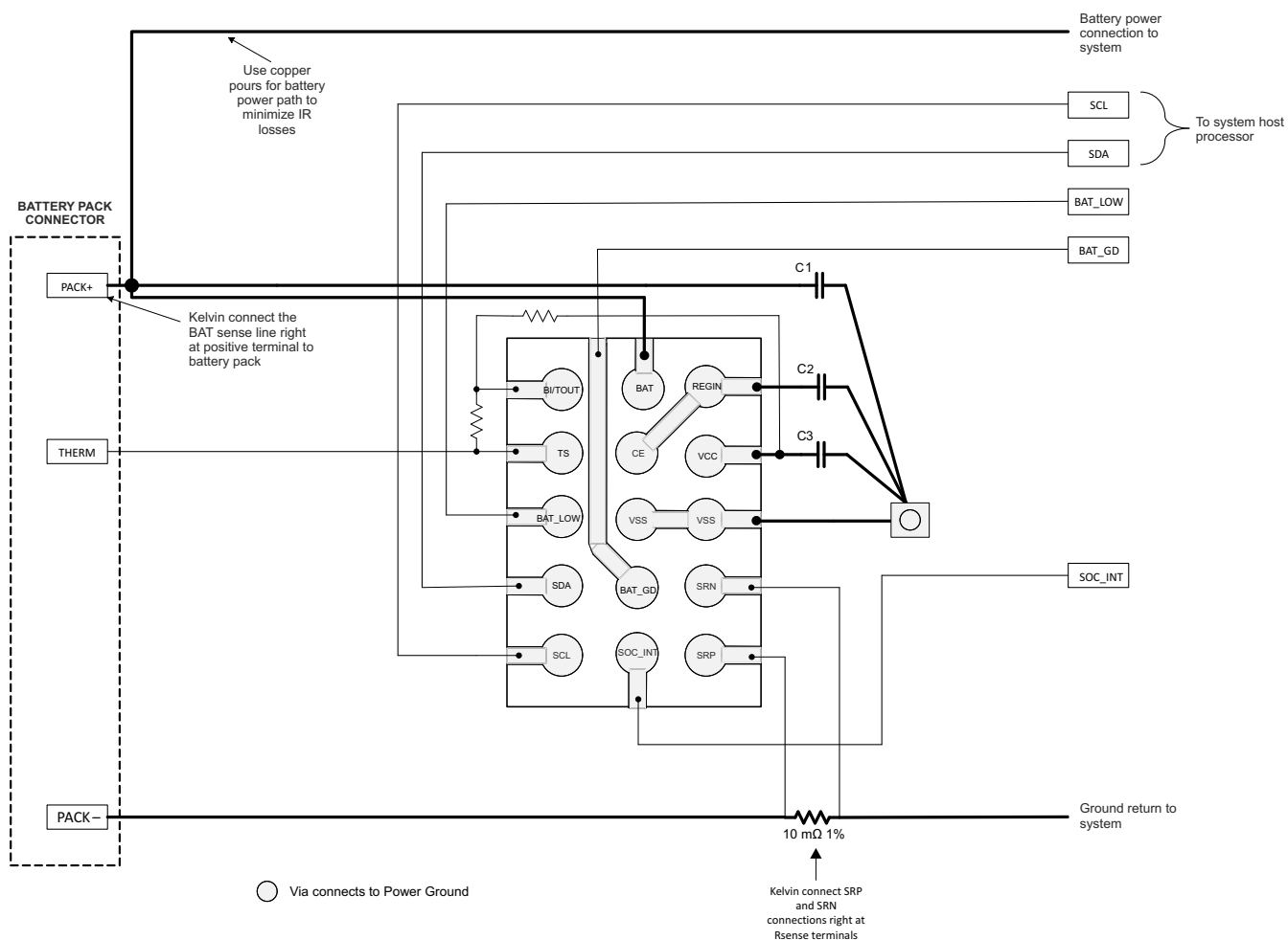
11-1. Layout Recommendation
