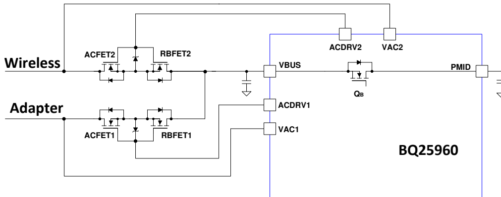
FIG 9-6. Two Inputs with ACFET-RBFET1 and ACFET-RBFET2
