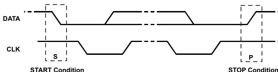
FIG 9-10. START and STOP Condition
