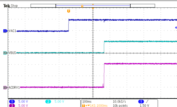
10-15. Power Up without AC-RFFET
