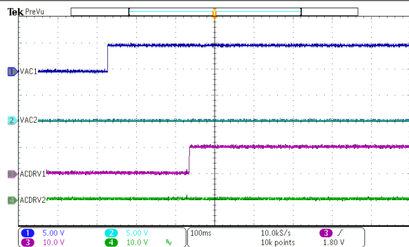
10-17. Power Up from VAC1 with ACFET1-RBFET1
