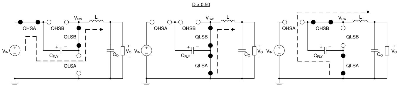
FIG 15. Three-Level Buck Converter States for Duty Ratios < 0.50
