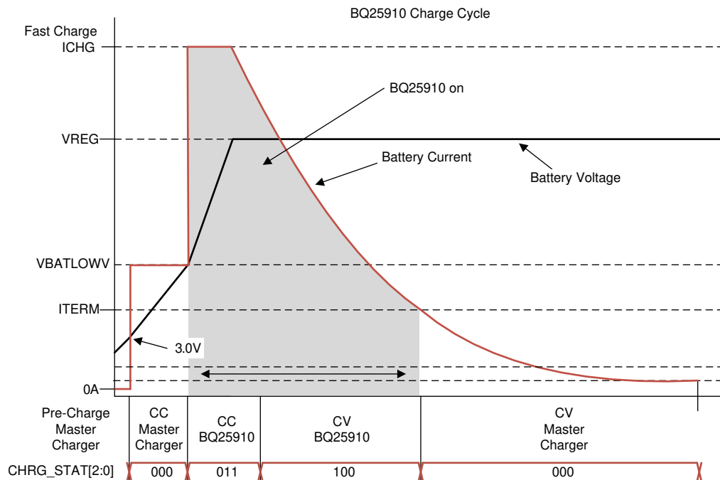
FIG 19. Battery Charging Profile Highlighting Parallel Charger Region of Operation
