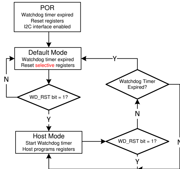
图 17. Watchdog Timer Flow Chart
