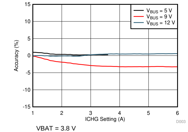
Figure 4. Charge Current Accuracy vs I²C ICHG Setting
