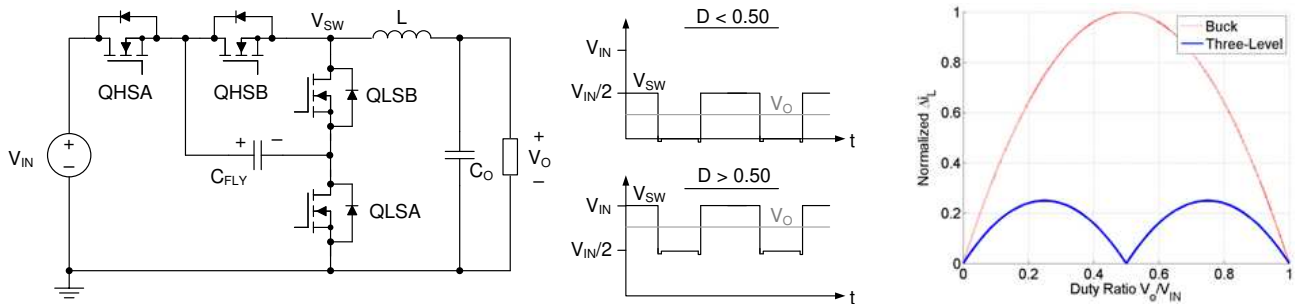
FIG 14. (a) Three-Level Buck Converter Circuit, (b) Time-Domain V_{SW} and V_O Waveforms, and (c) Inductor Current Ripple Comparison Across Duty Ratio
