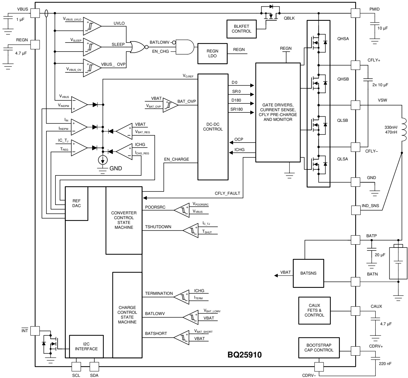
FIG 13. BQ25910 I²C Controlled Functional Block Diagram
