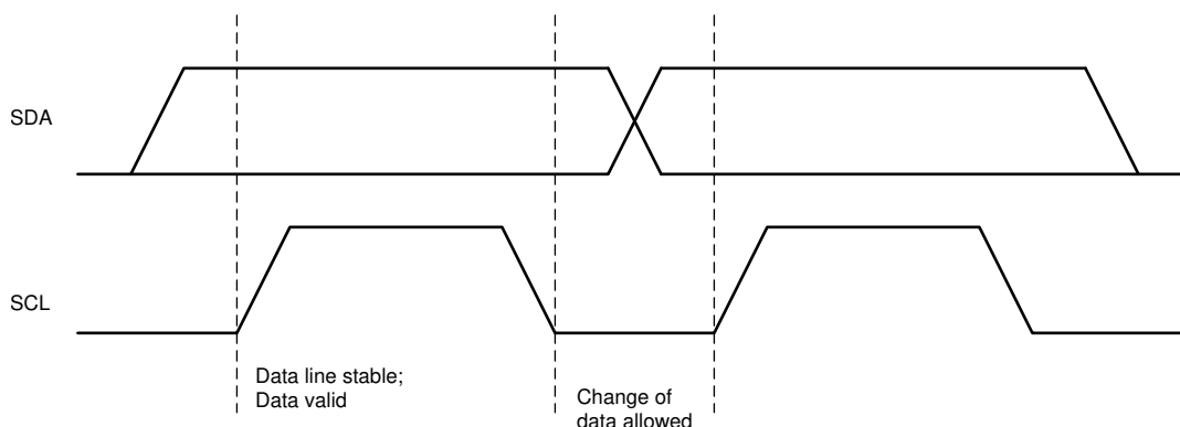
✎ 22. Bit Transfers on the I 2 C Bus
