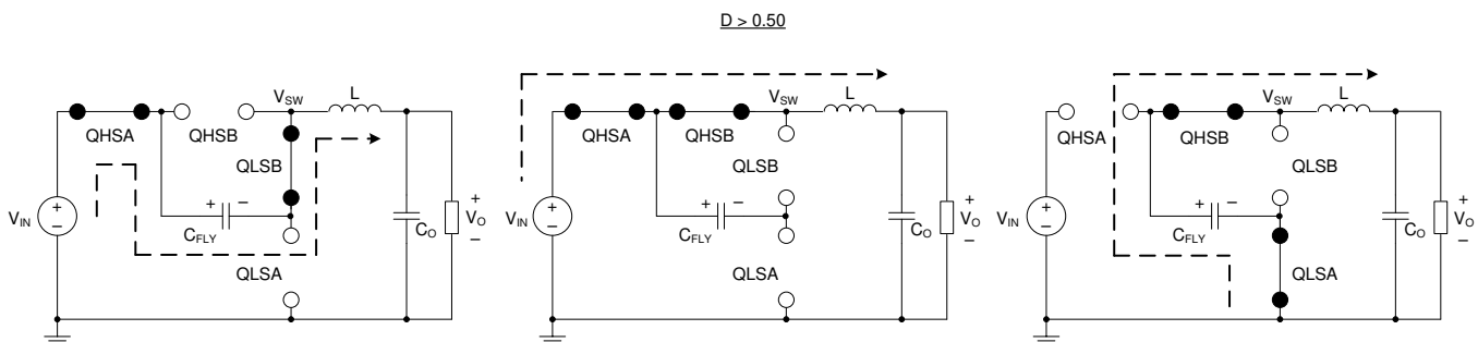
FIG 16. Three-Level Buck Converter States for Duty Ratios > 0.50
