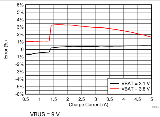
8-4. Charge Current Accuracy vs Charge Current I 2 C Setting
