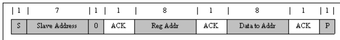
FIG 19. Single Write
