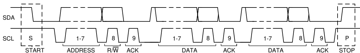
FIG 18. Complete Data Transfer on the I2C Bus
