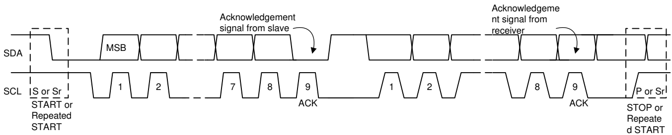
FIG 16. Data Transfer on the I2C Bus
