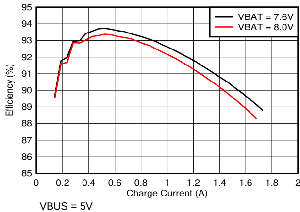
FIG 1. Charge Efficiency vs. Charge Current
