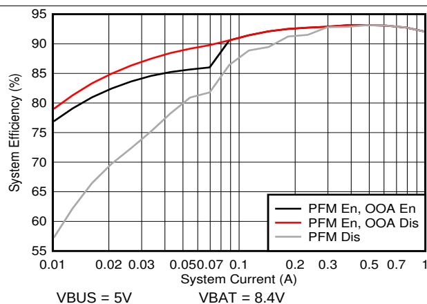
FIG 5. System Efficiency vs. System Current
