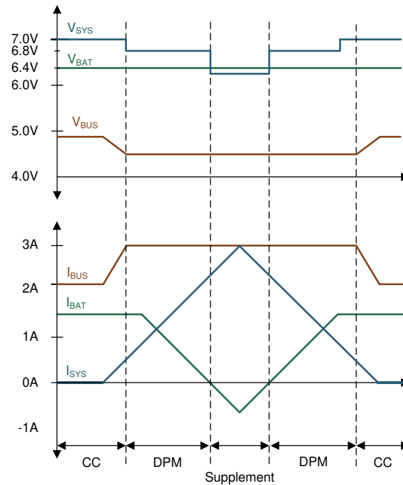
FIG 20. DPM Response
