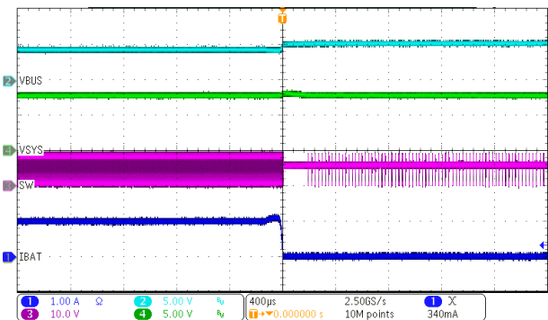
Figure 77. Adapter Power Up With Charge Enabled
