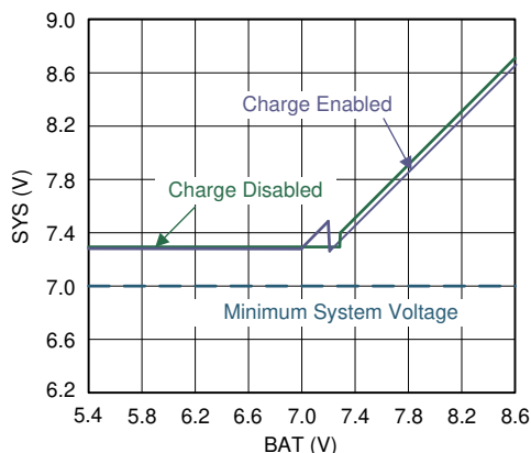
FIG 19. System Voltage vs. Battery Voltage
