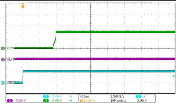
Figure 79. Charge Disable
