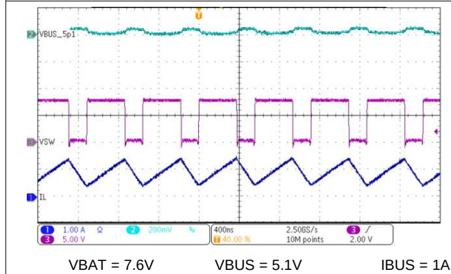
图 84. Buck Mode (OTG) PWM Switching
