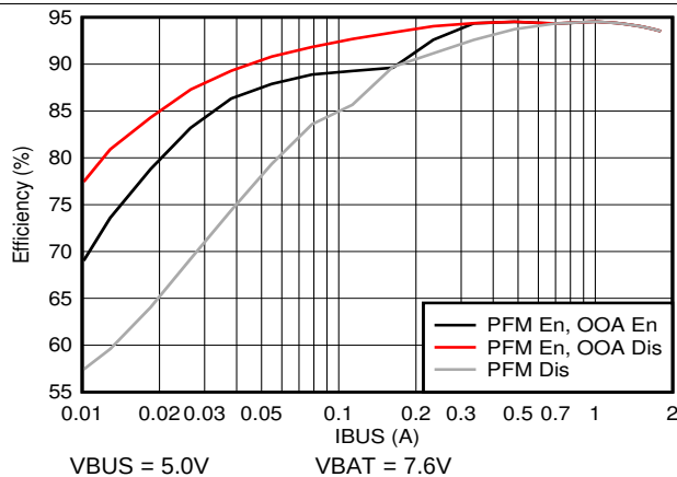
FIG 3. OTG Efficiency vs. VBUS Output Current
