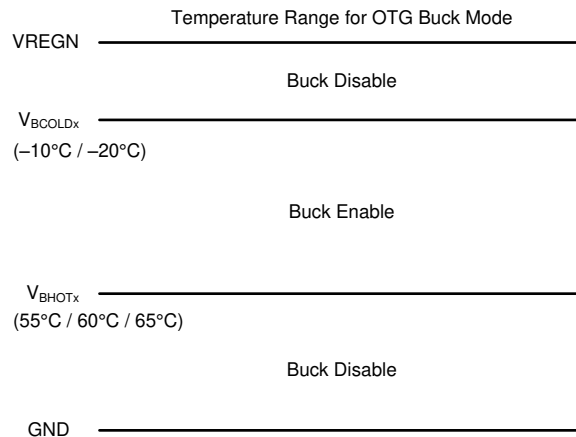
FIG 25. TS Pin Thermistor Sense Threshold in OTG Buck Mode
