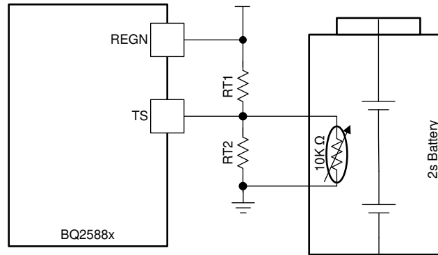
FIG 23. TS Resistor Network
