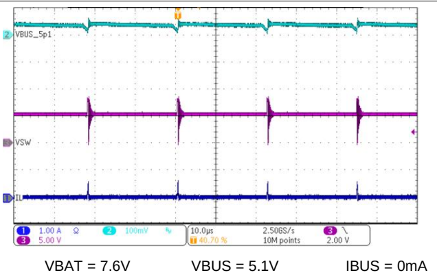
图 85. Buck Mode (OTG) PFM Switching
