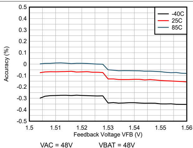
FIG 6-4. Feedback Voltage Accuracy (at different temperatures)
