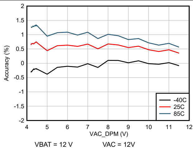
Figure 6-7. Input Voltage (VAC_DPM) Regulation Accuracy (at different temperatures)
