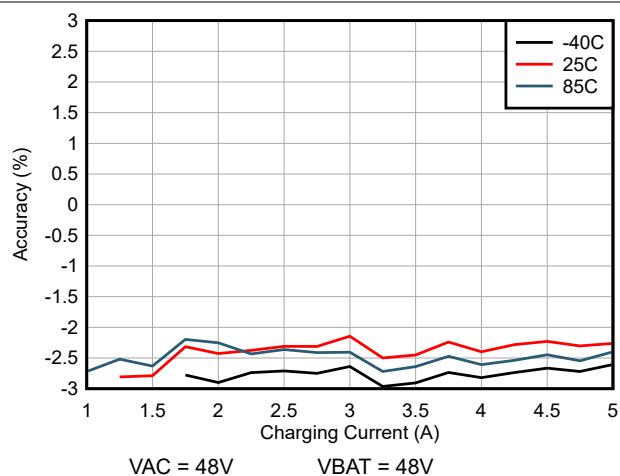
FIG 6-6. Charge Current Accuracy (at different temperatures)
