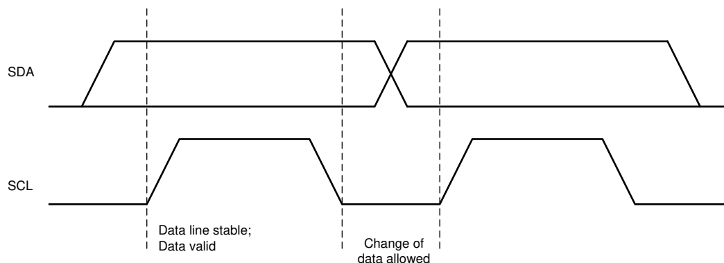
✎ 7-7. Bit Transfers on the I 2 C Bus
