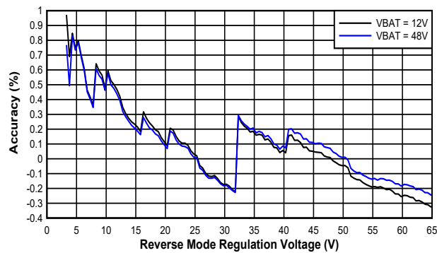
6-13. Reverse Mode Output Voltage Accuracy vs VAC_REV Setting
