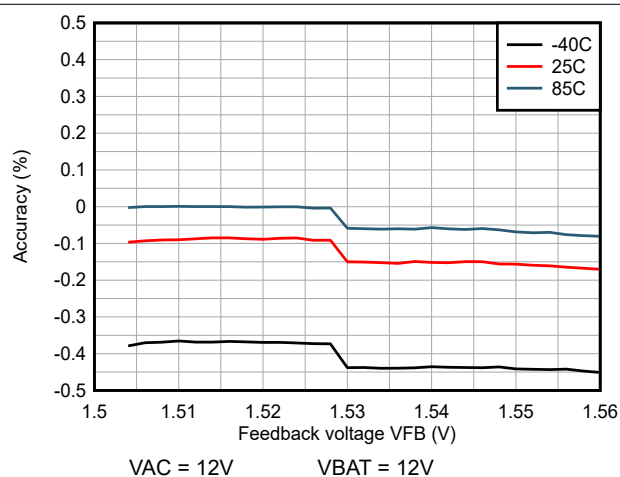
FIG 6-3. Feedback Voltage Accuracy (at different temperatures)
