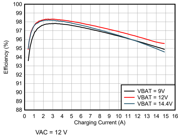
6-1. Charge Efficiency vs Charge Current (4s LiFePO4 battery configuration)
