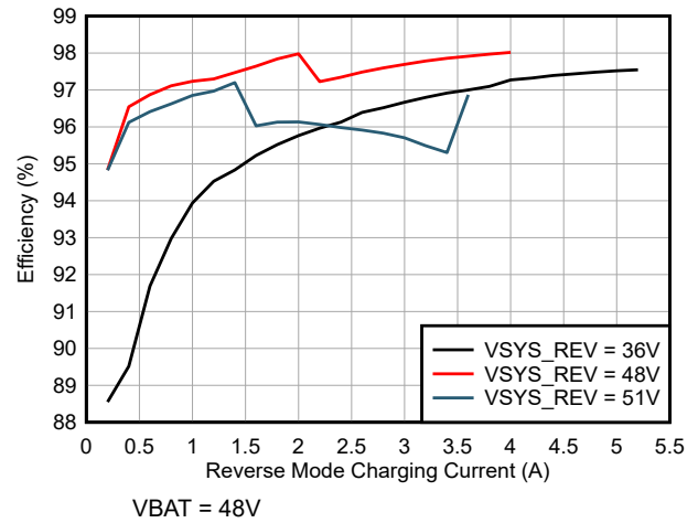
6-12. Reverse Mode Efficiency (12s Li-Ion battery configuration)
