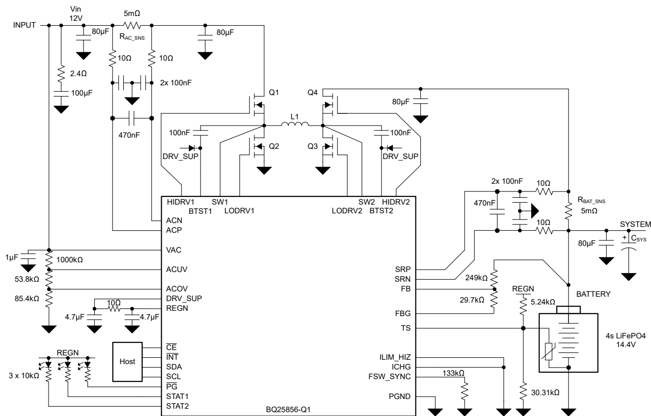
8-13. BQ25856-Q1: Bi-directional Charging From a 12V Input to Charge a 4s LiFePO 4 Car Battery
