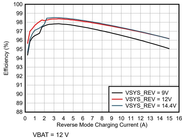
6-11. Reverse Mode Efficiency (4s LiFePO4 battery configuration)
