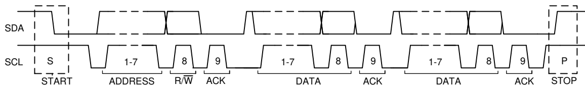
图 7-10. Complete Data Transfer on the I 2 C Bus
