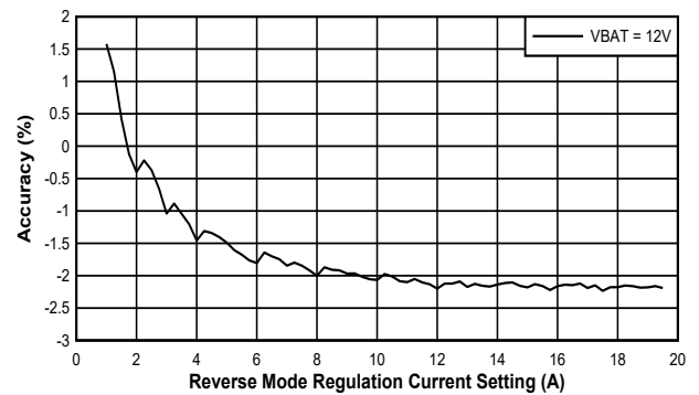
6-14. Reverse Mode Output Current Accuracy vs IAC_REV Setting
