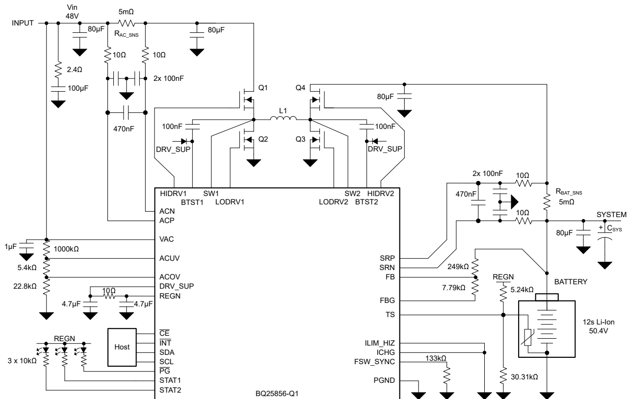
8-1. BQ25856-Q1: Bi-directional Charging From a 48V Input to Charge a 12s Li-Ion Car Battery
