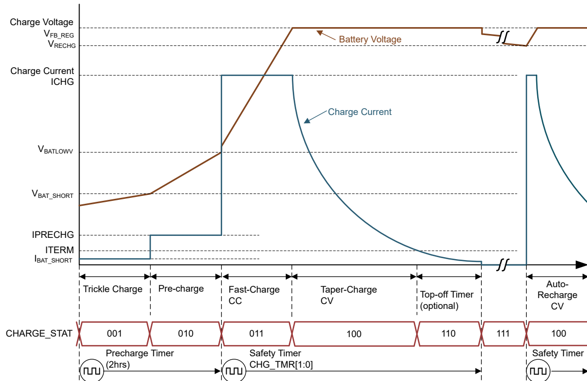
図 7-3. Typical Li-Ion Battery Charging Profile
