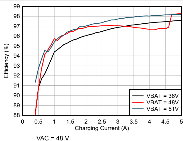
FIG 6-2. Charge Efficiency vs Charge Current
