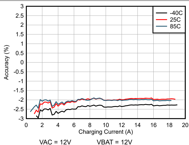
FIG 6-5. Charge Current Accuracy (at different temperatures)
