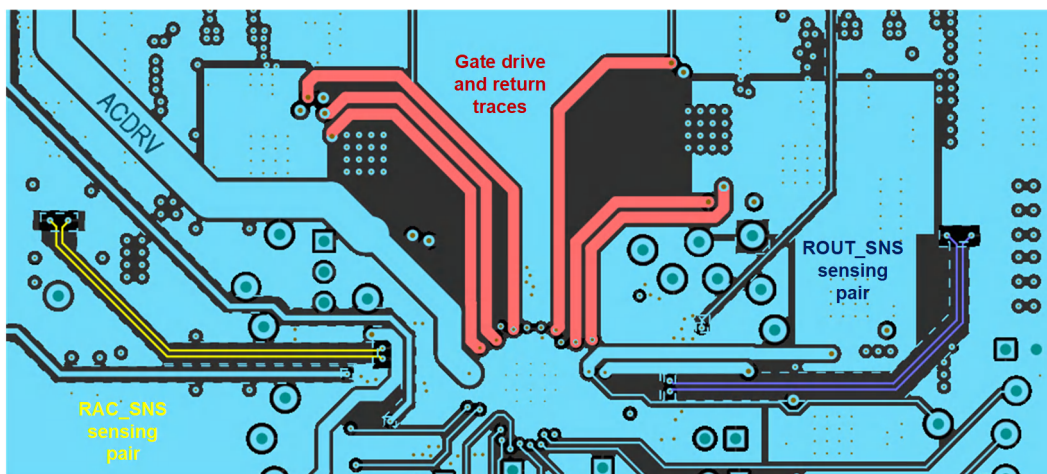
図 10-2. PCB Layout Gate Drive and Current Sensing Signal Layer Routing
