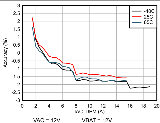
Figure 6-9. Input Current (IAC_DPM) Regulation Accuracy (at different temperatures)
