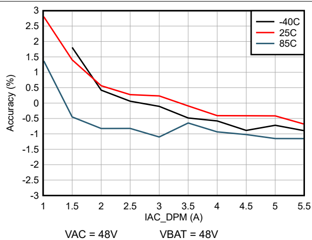
Figure 6-10. Input Current (IAC_DPM) Regulation Accuracy (at different temperatures)
