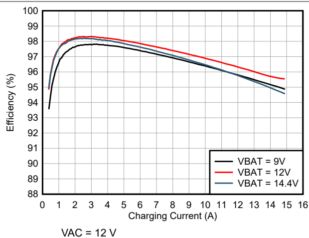
FIG 6-1. Charge Efficiency vs Charge Current (4s LiFePO4 battery configuration)
