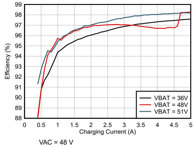
6-2. Charge Efficiency vs Charge Current
