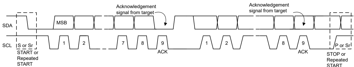
図 7-9. Data Transfer on the I 2 C Bus
