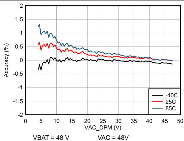
Figure 6-8. Input Voltage (VAC_DPM) Regulation Accuracy (at different temperatures)
