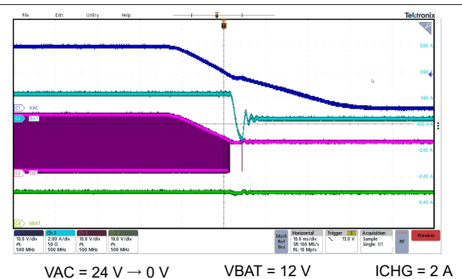
図 8-4. VAC Un-plug Power Down with 2-A ICHG
