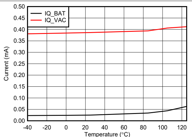
図 6-6. Battery and Input Quiescent Current vs Temperature with VBAT = 20 V
