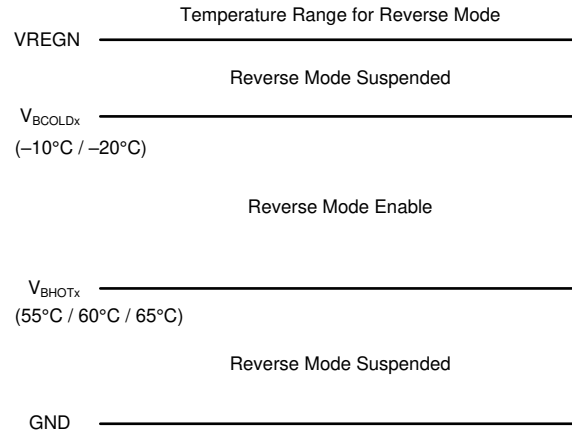
图 7-5. TS Pin Thermistor Sense Threshold in Reverse Mode
