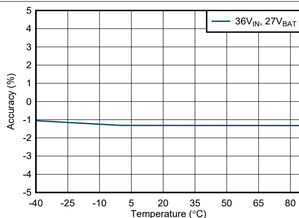
図 6-5. Charge Current Accuracy vs Temperature
