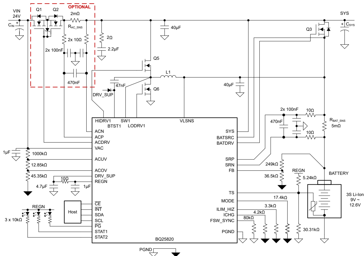
図 8-1. BQ25820: I 2 C Controlled, 24 VAC with 3-S Li-Ion Battery, 10-A Charge Current and 350-kHz Switching Frequency
