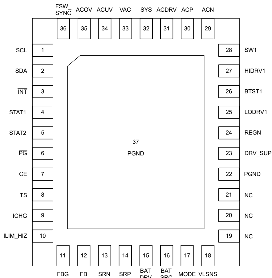
図 5-1. BQ25820, RRV Package 36-pin VQFN Top View
