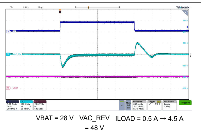
図 8-8. Reverse Mode Boost Transient Reponse
