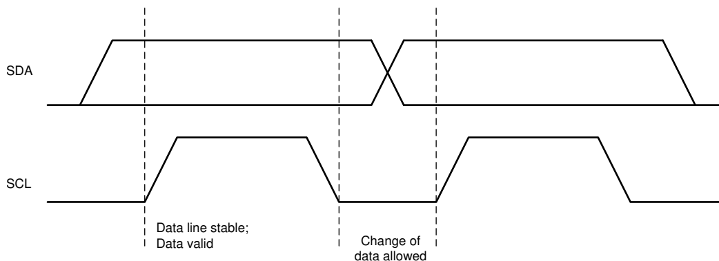
図 7-7. Bit Transfers on the I 2 C Bus
