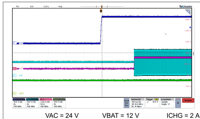
図 8-3. VAC Plug-In Power Up with 2-A ICHG
