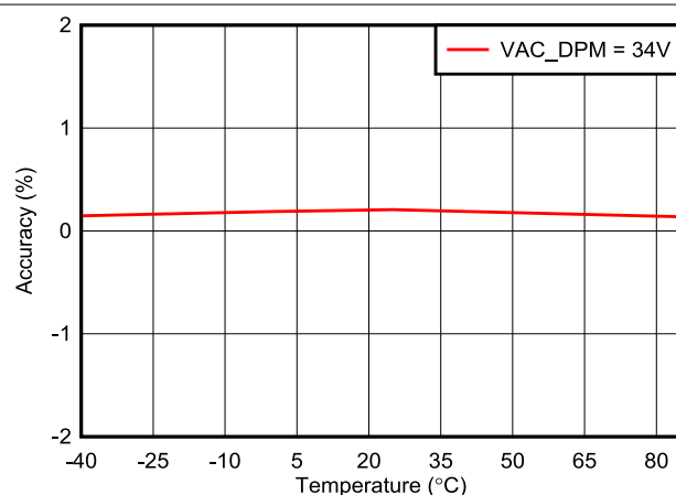
図 6-7. Input Voltage (VAC_DPM) Regulation Accuracy vs Temperature
