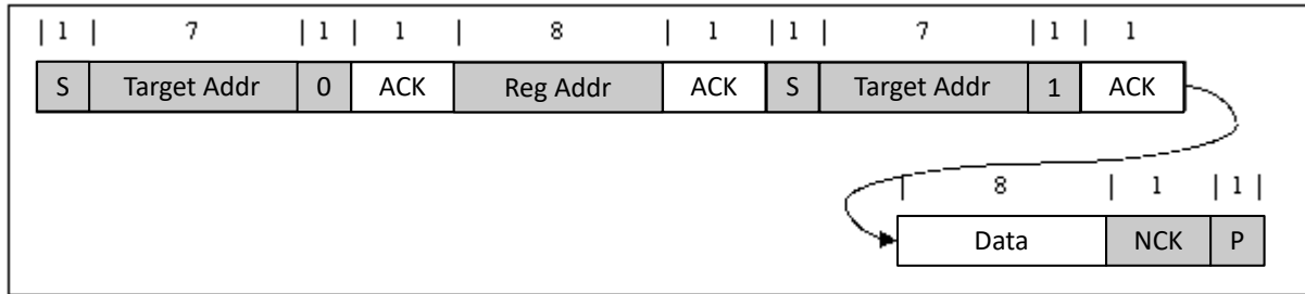
図 7-12. Single Read
