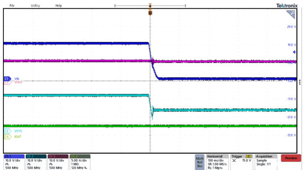
図 8-9. VAC to VBAT Power Path Transfer
