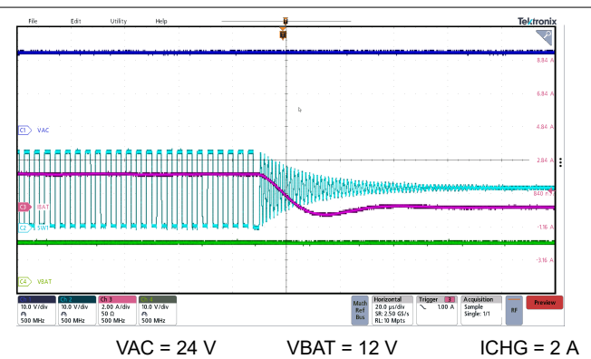
図 8-6. Charge Disable via I 2 C with 2-A ICHG
