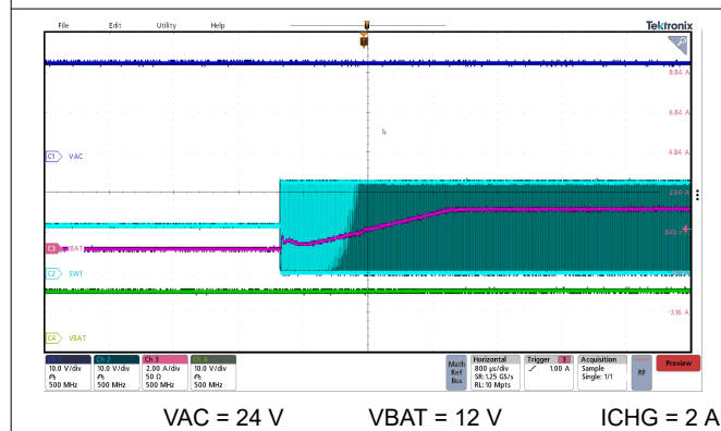
図 8-5. Charge Enable via I 2 C with 2-A ICHG
