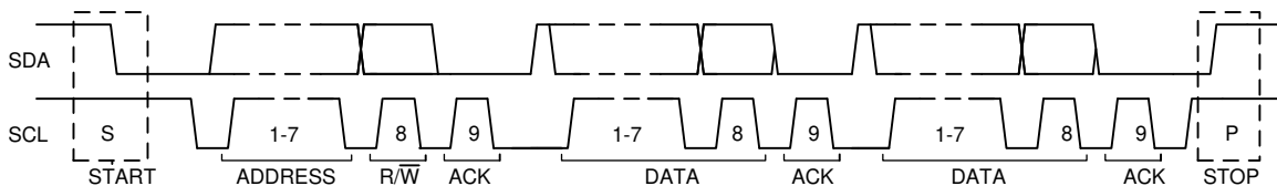
図 7-10. Complete Data Transfer on the I 2 C Bus
