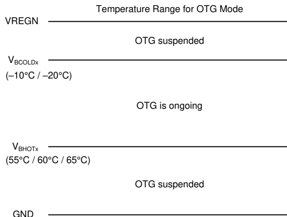
FIG 9-13. TS Pin Thermistor Sense Threshold in OTG Mode
