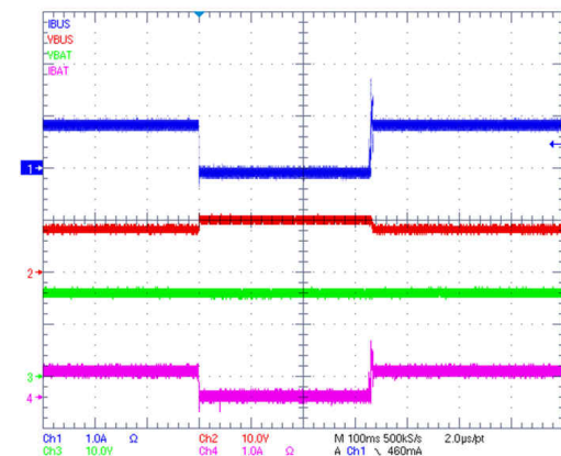
10-17. VOTG Load Transient Response
