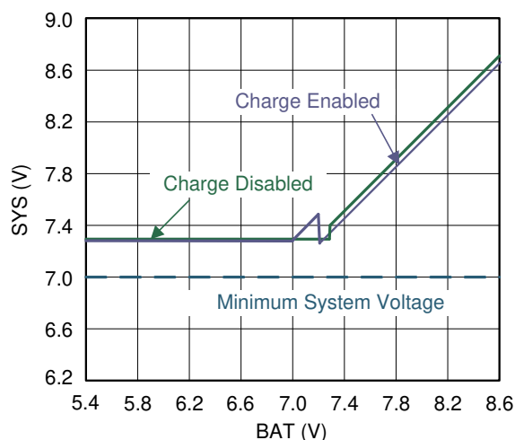
FIG 9-7. Typical System Voltage vs Battery Voltage for a 2S Battery Configuration
