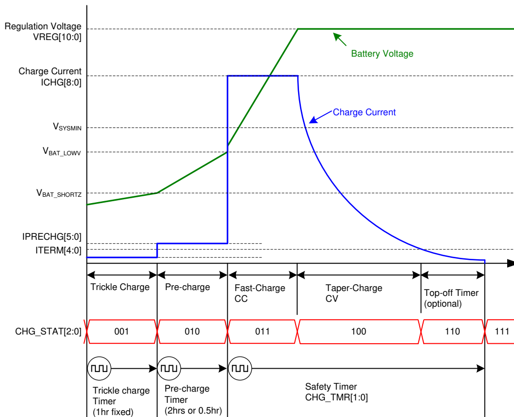
FIG 9-10. Battery Charging Profile
