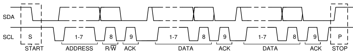
FIG 9-20. Complete Data Transfer on the I 2 C Bus
