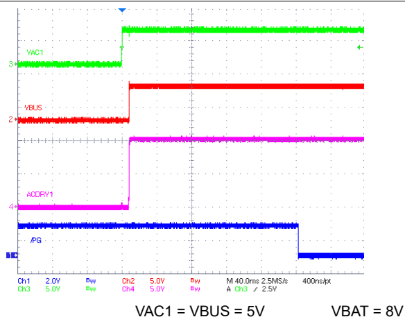
10-4. ACFET1-RBFET1 Turns on at Power Up
