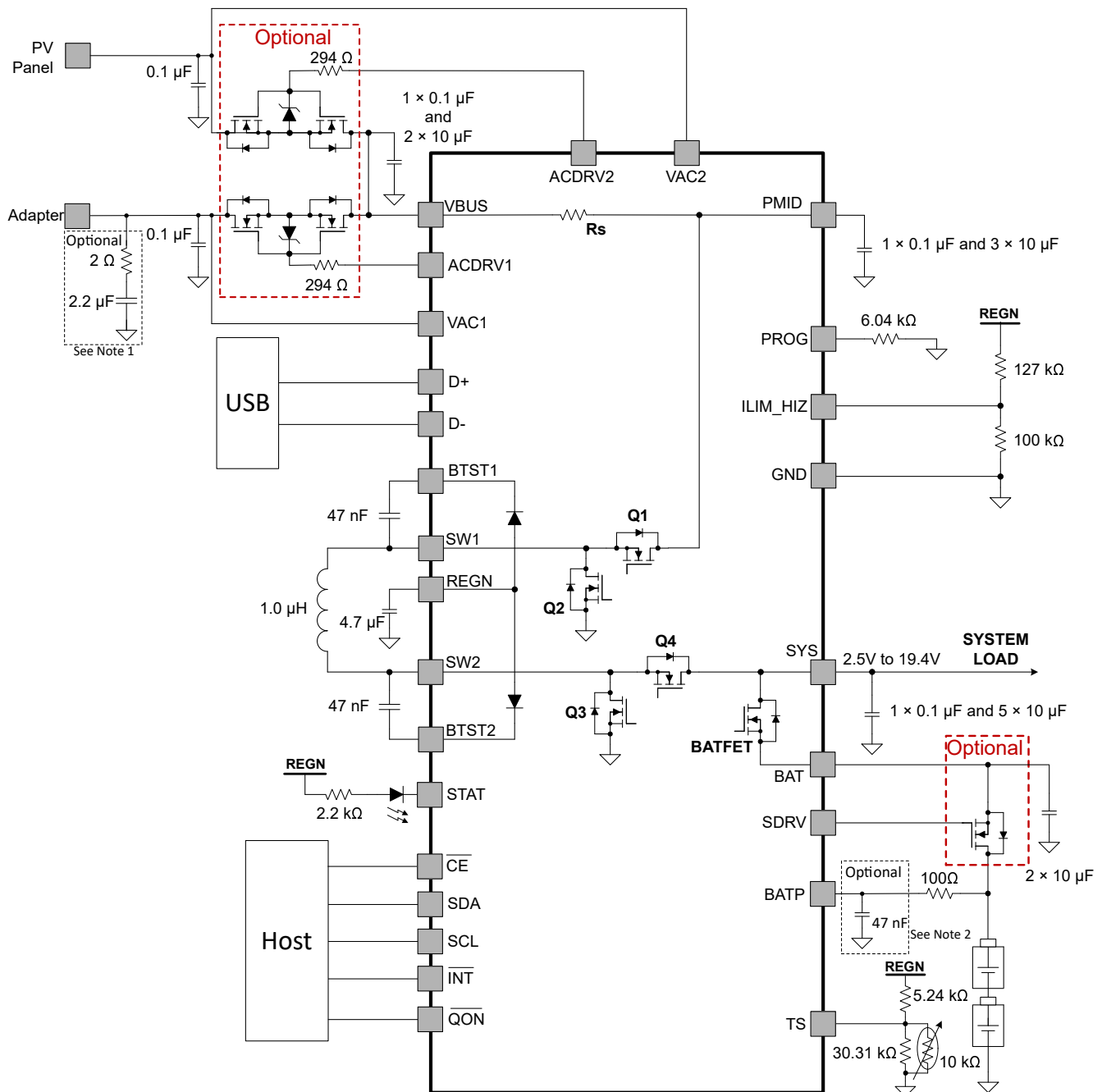
FIG 10-1. BQ25798 Application Diagram with Two Input Sources and Ship FET
