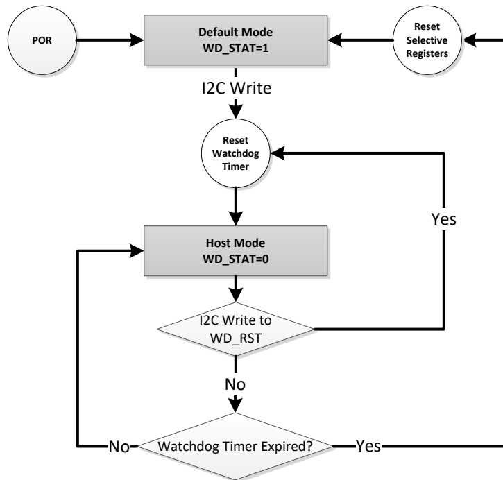
FIG 9-25. Watchdog Timer Flow Chart
