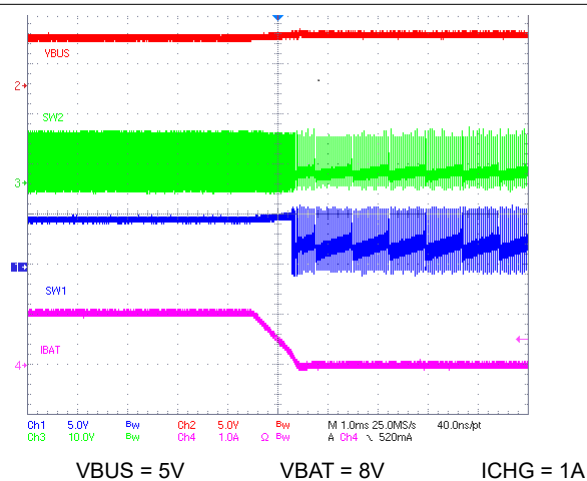
10-7. Charge Disable
