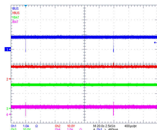
10-16. IINDPM Transient Response
