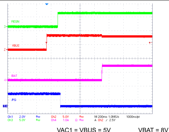
10-5. Power Up from VAC1 with Charge Enabled
