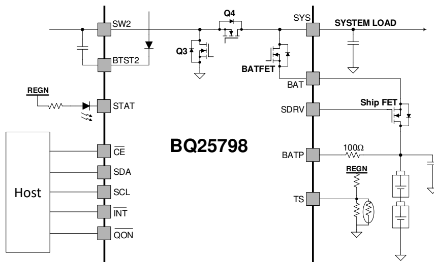
FIG 9-15. The Application Diagram for the External Ship FET
