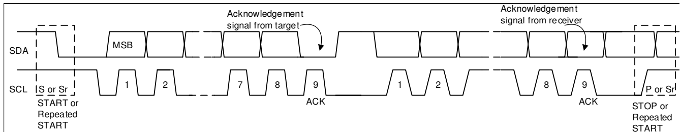
FIG 9-18. Data Transfer on the I 2 C Bus
