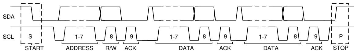
FIG 9-19. Complete Data Transfer on the I 2 C Bus
