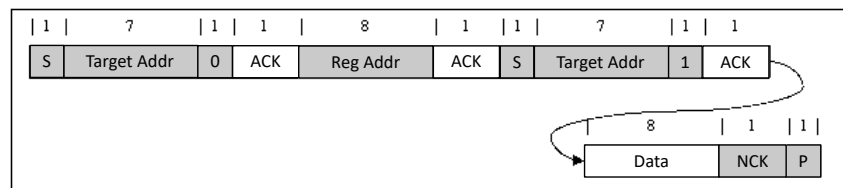
FIG 9-21. Single Read
