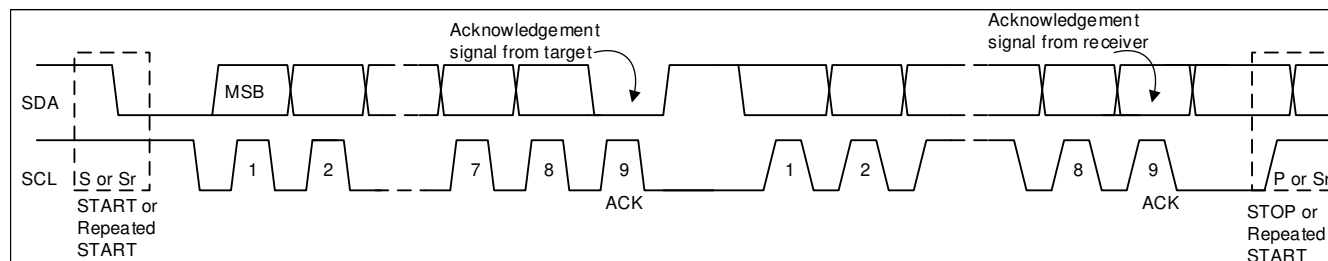
FIG 9-17. Data Transfer on the I 2 C Bus
