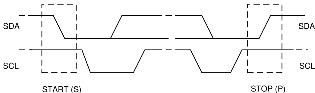
FIG 9-16. START and STOP Conditions on the I 2 C Bus
