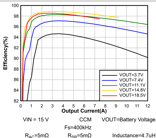
8-3. Charge Efficiency
