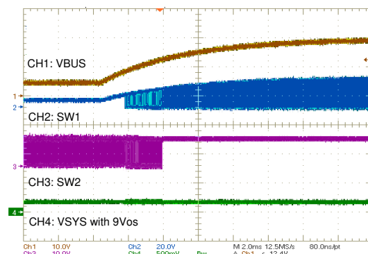
FIG 10-5. Power Up From 5 V
