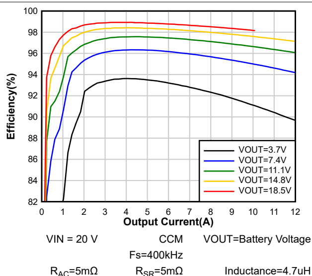
8-4. Charge Efficiency
