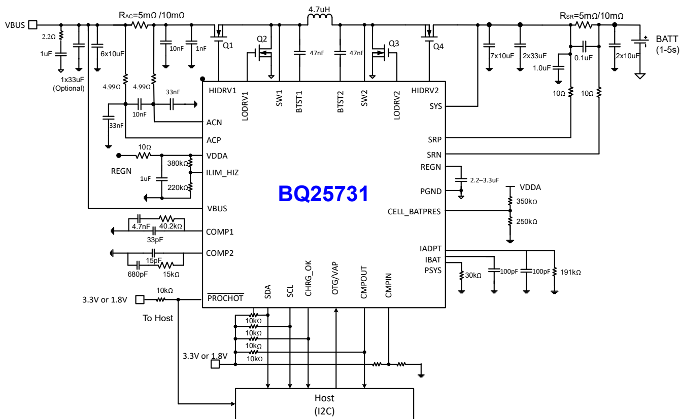
10-1. Application Diagram of BQ25731 with Non Power Path
