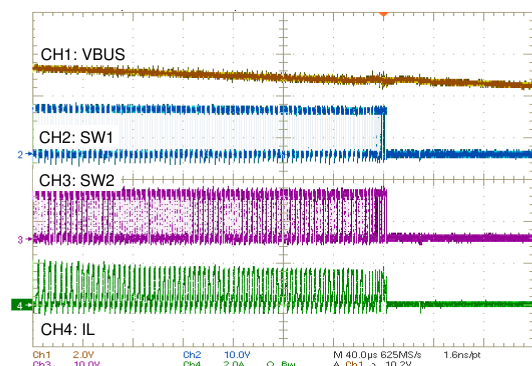
FIG 10-4. Power Up From 20 V
