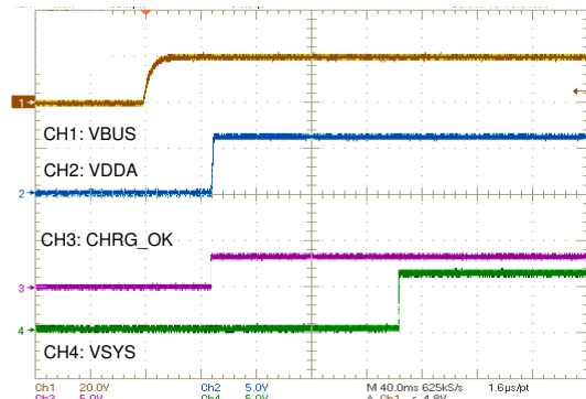
FIG 10-4. Power Up From 20 V
