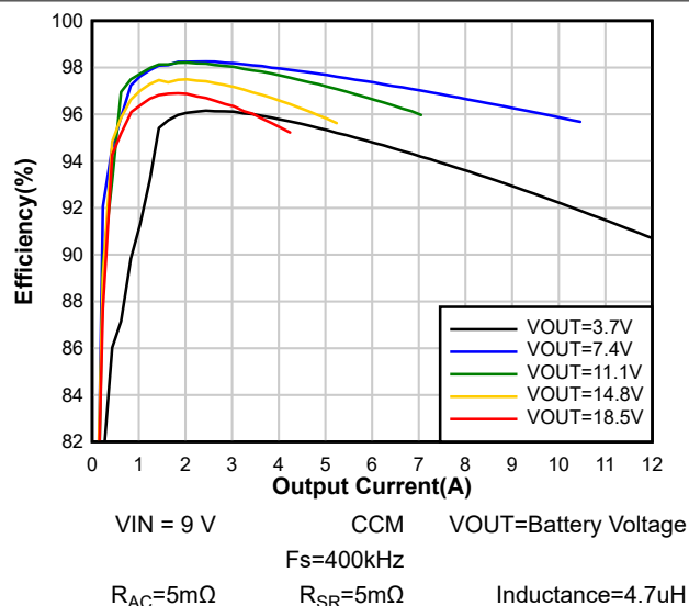
8-2. Charge Efficiency
