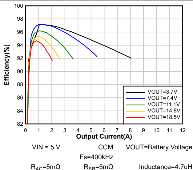
8-1. Charge Efficiency
