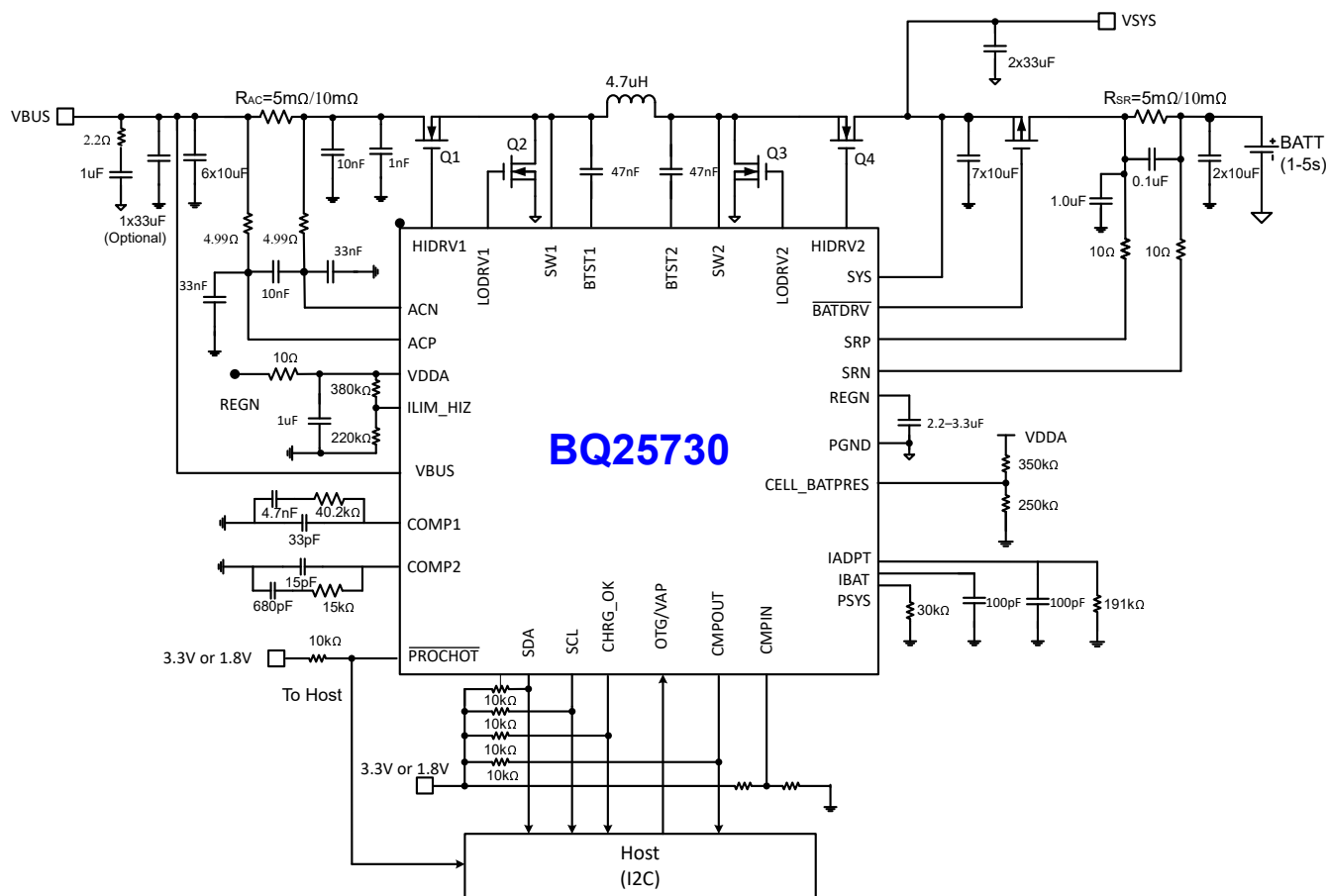
9-1. Application Diagram of BQ25730 with Power Path
