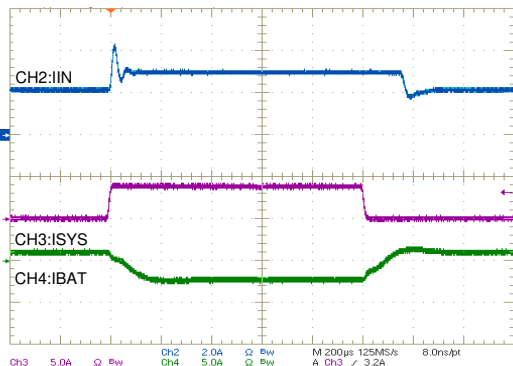
図 9-16. Input Current in Boost Mode
