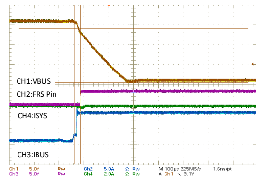
図 9-21. FRS Transition Waveform
