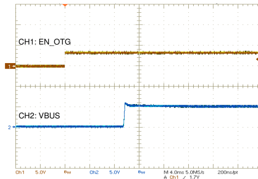
図 9-17. OTG Power Up from 8-V Battery
