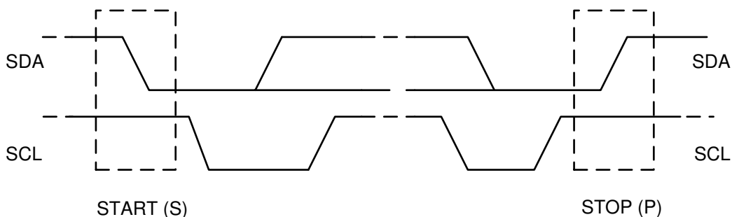
✎ 8-16. START and STOP Conditions on the I²C Bus
