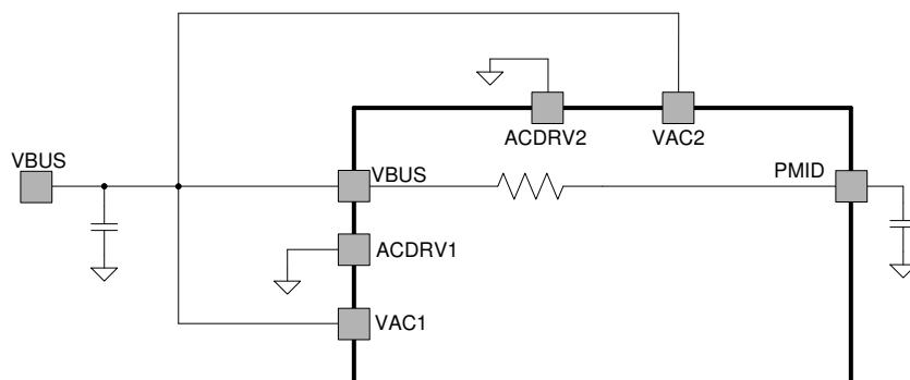
✎ 8-2. Single Input Connected to VBUS Directly Without ACFET-RBFET
