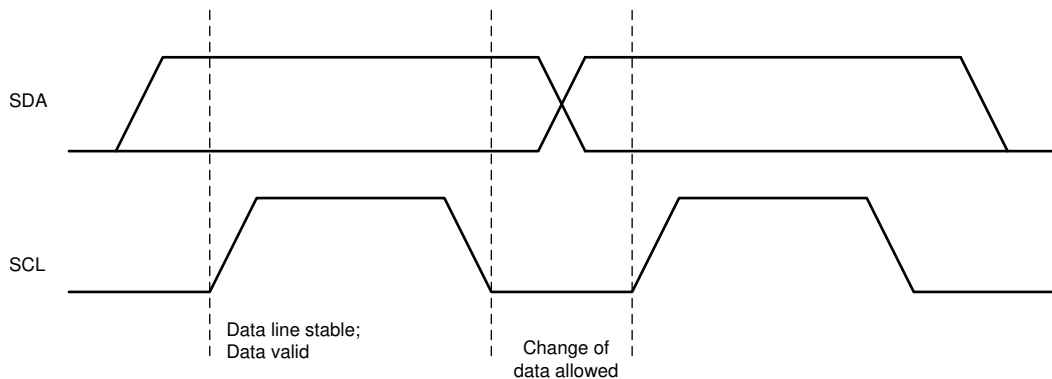
✎ 8-15. Bit Transfers on the I²C Bus
