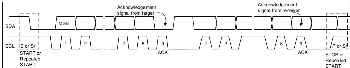
✎ 8-17. Data Transfer on the I²C Bus
