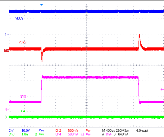
图 9-5. OTG Startup at No Load
