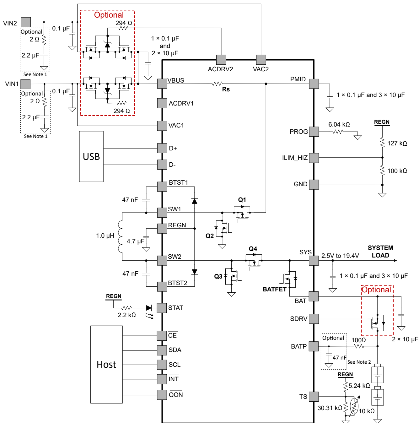
FIG 9-1. BQ25672 Application Diagram with Two Input Sources and Ship FET
