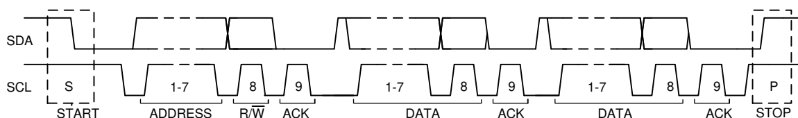
8-19. Complete Data Transfer on the I 2 C Bus
