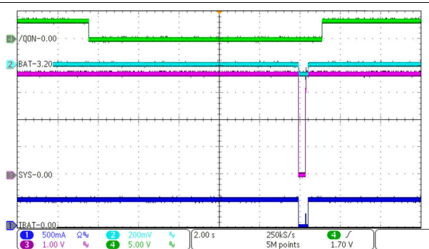
図 9-5. Charge Disable
