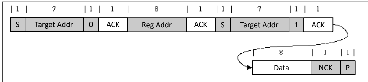
図 8-12. Single Read
